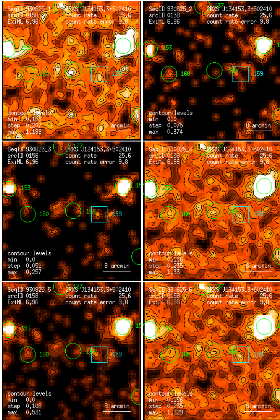
Figure 158: RASS 930825: detection 0158: band rate images, Gaussian filter: (1) PSPC channels 11 – 41, (2) 52 – 90, (3) 91 – 201, (4) 11 – 235, (5) 52 – 201, (6) 11 – 201. Broad band rates in counts/ks. Band rate contour levels in counts/ks/arcmin 2 .
