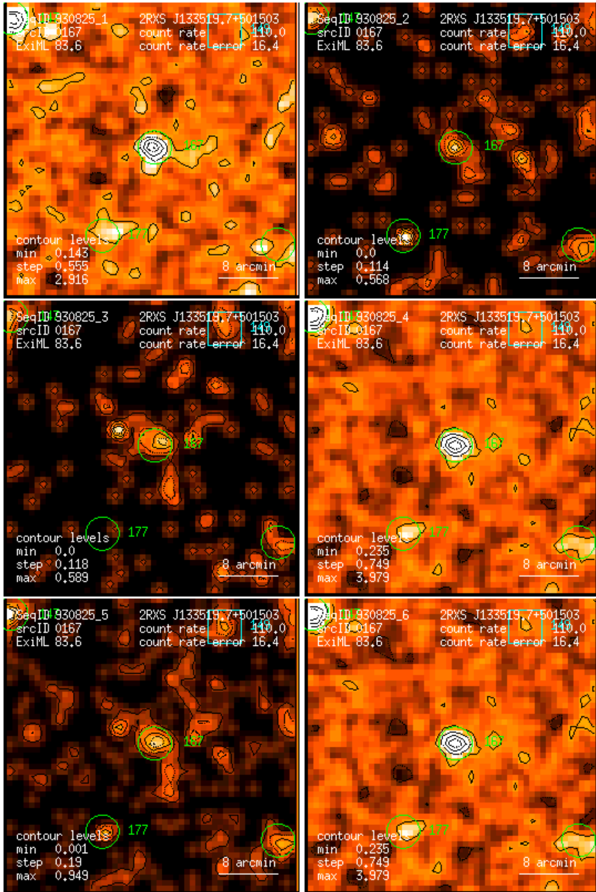
Figure 167: RASS 930825: detection 0167: band rate images, Gaussian filter: (1) PSPC channels 11 – 41, (2) 52 – 90, (3) 91 – 201, (4) 11 – 235, (5) 52 – 201, (6) 11 – 201. Broad band rates in counts/ks. Band rate contour levels in counts/ks/arcmin 2 .
