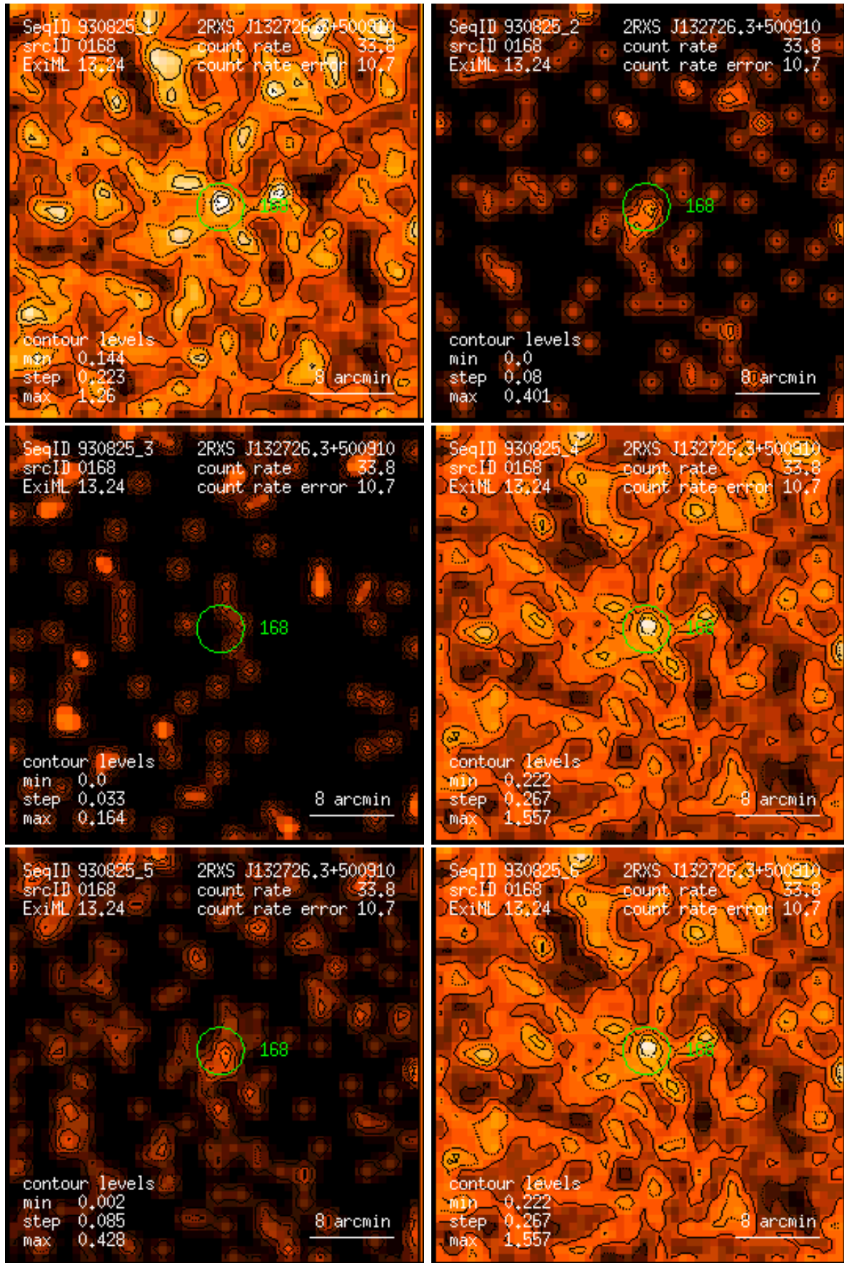
Figure 168: RASS 930825: detection 0168: band rate images, Gaussian filter: (1) PSPC channels 11 – 41, (2) 52 – 90, (3) 91 – 201, (4) 11 – 235, (5) 52 – 201, (6) 11 – 201. Broad band rates in counts/ks. Band rate contour levels in counts/ks/arcmin 2 .
