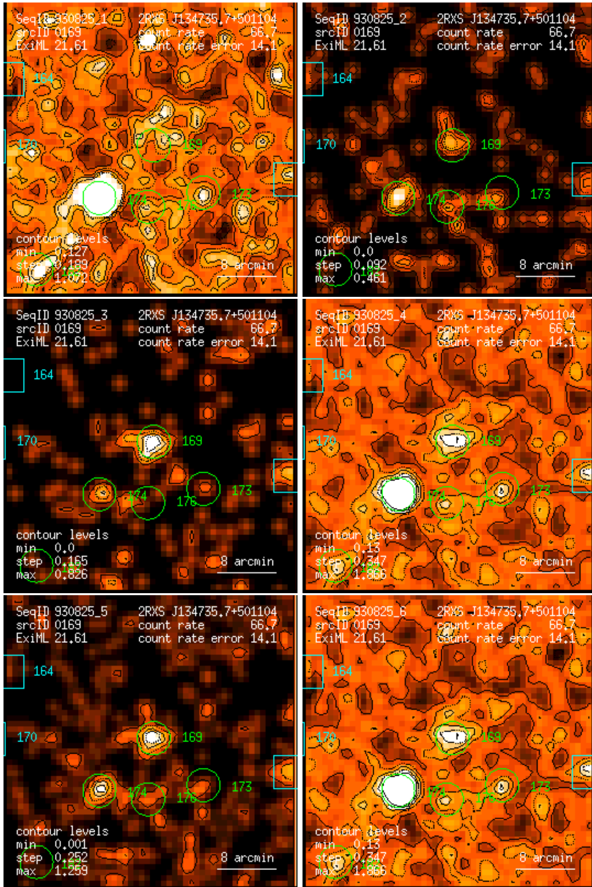
Figure 169: RASS 930825: detection 0169: band rate images, Gaussian filter: (1) PSPC channels 11 – 41, (2) 52 – 90, (3) 91 – 201, (4) 11 – 235, (5) 52 – 201, (6) 11 – 201. Broad band rates in counts/ks. Band rate contour levels in counts/ks/arcmin 2 .
