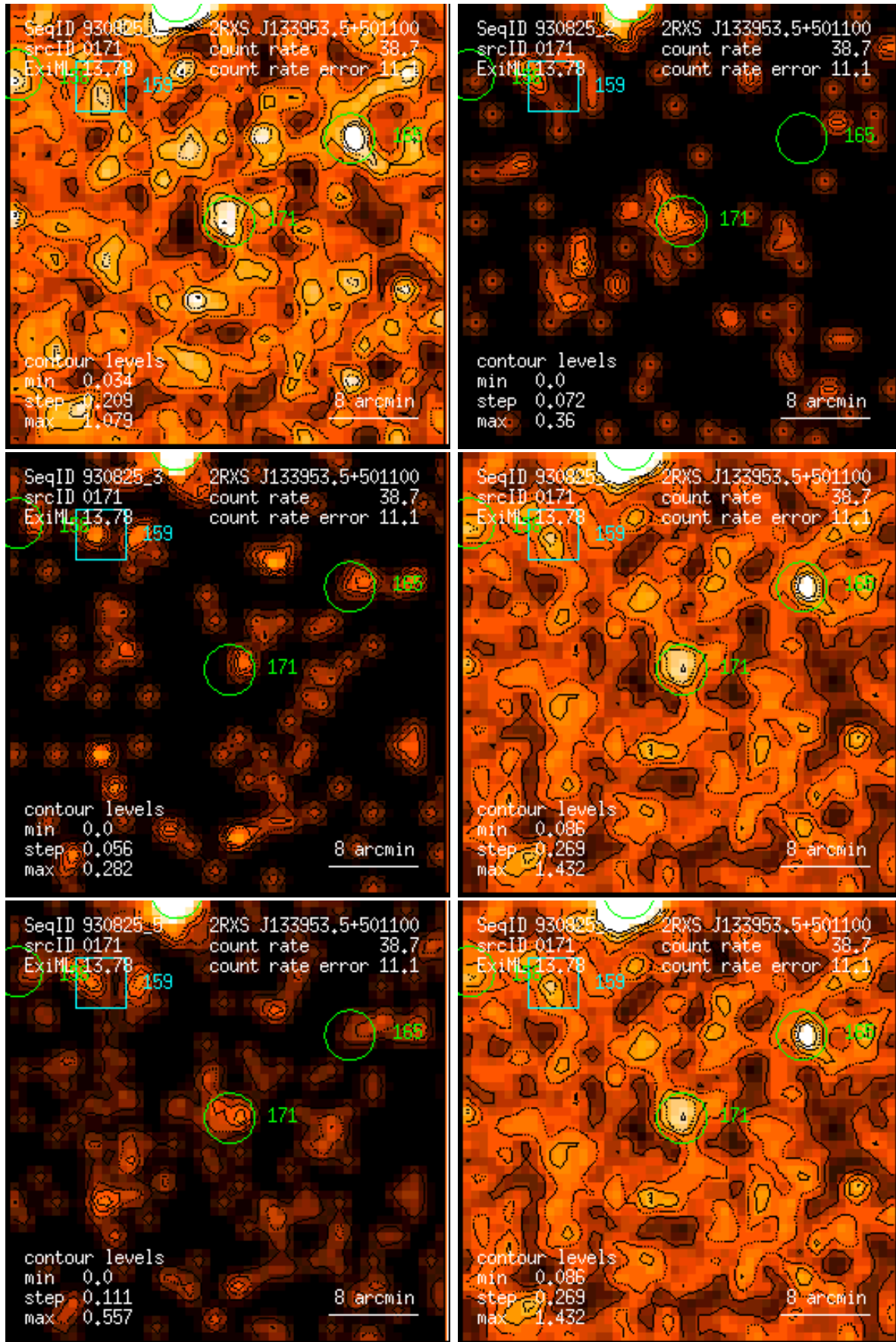
Figure 171: RASS 930825: detection 0171: band rate images, Gaussian filter: (1) PSPC channels 11 – 41, (2) 52 – 90, (3) 91 – 201, (4) 11 – 235, (5) 52 – 201, (6) 11 – 201. Broad band rates in counts/ks. Band rate contour levels in counts/ks/arcmin 2 .
