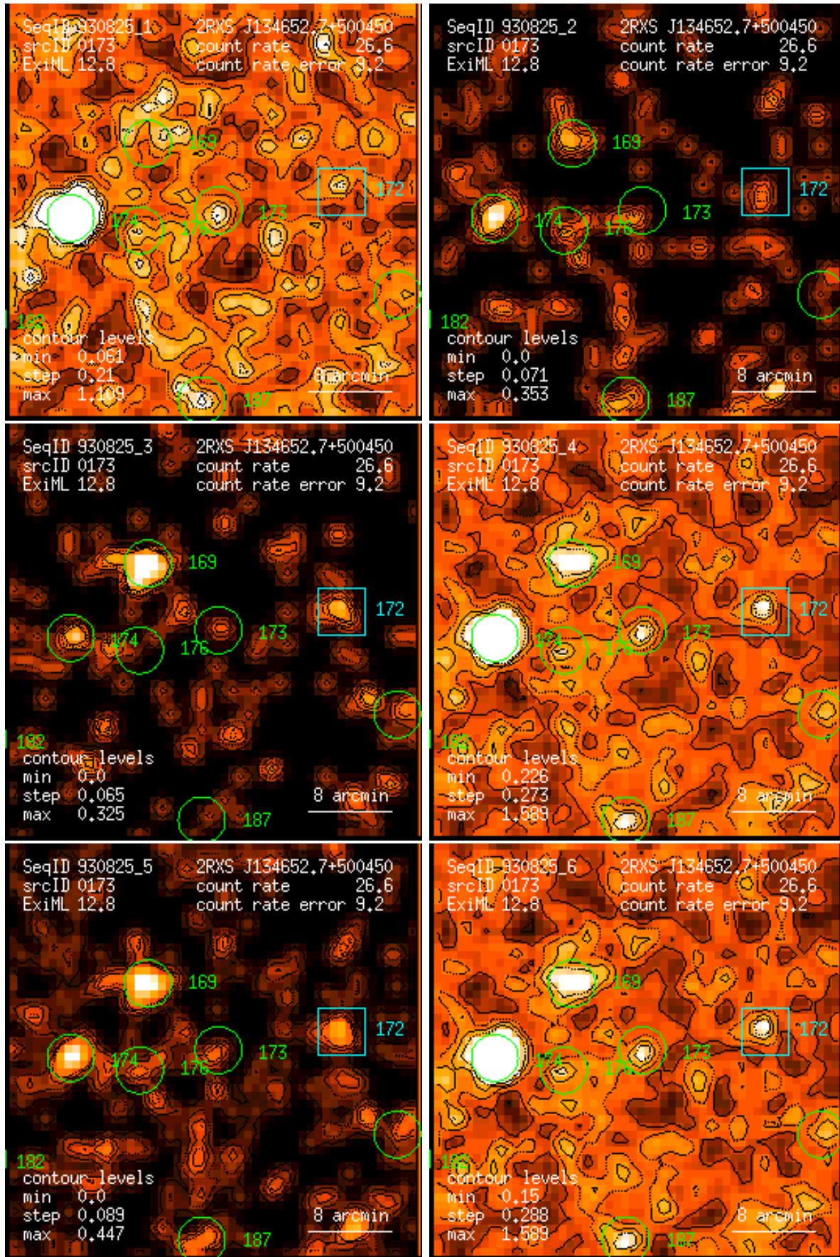
Figure 173: RASS 930825: detection 0173: band rate images, Gaussian filter: (1) PSPC channels 11 – 41, (2) 52 – 90, (3) 91 – 201, (4) 11 – 235, (5) 52 – 201, (6) 11 – 201. Broad band rates in counts/ks. Band rate contour levels in counts/ks/arcmin 2 .
