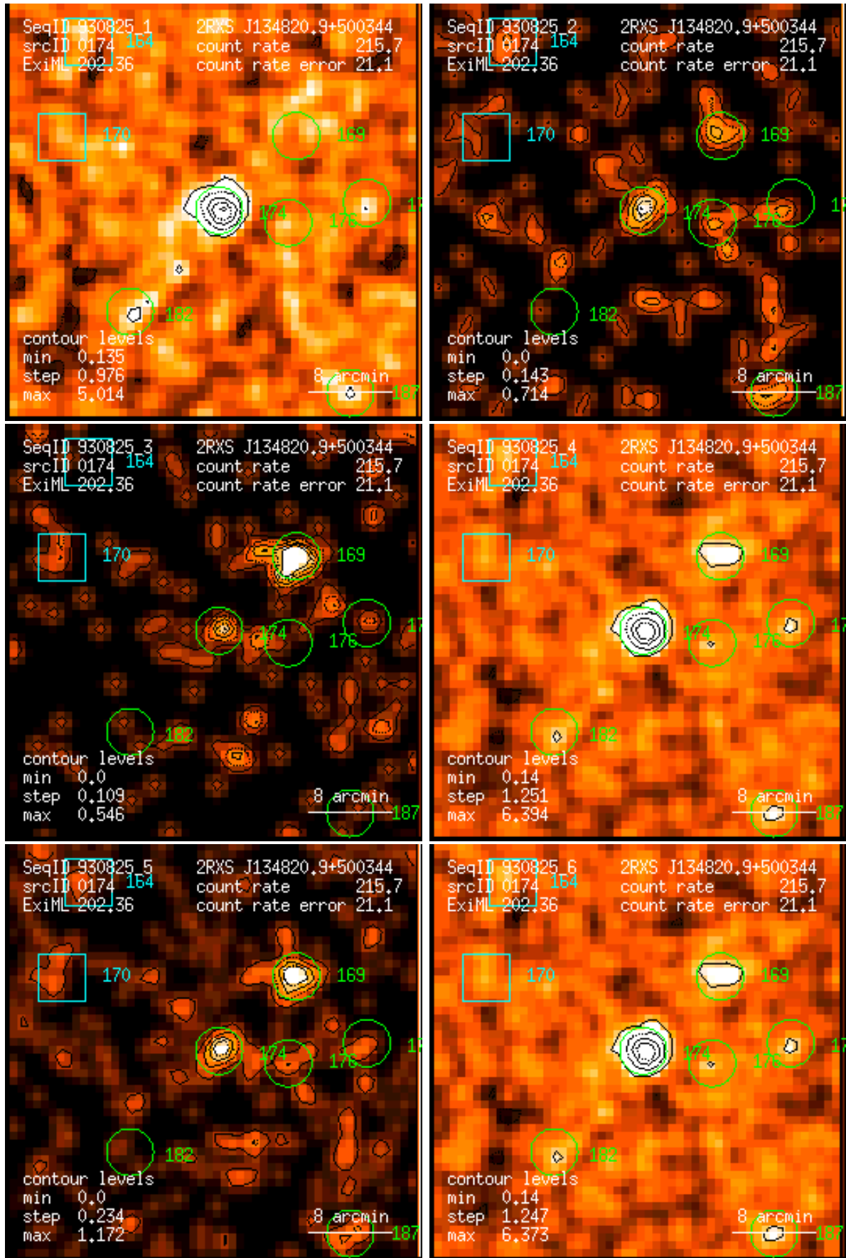
Figure 174: RASS 930825: detection 0174: band rate images, Gaussian filter: (1) PSPC channels 11 – 41, (2) 52 – 90, (3) 91 – 201, (4) 11 – 235, (5) 52 – 201, (6) 11 – 201. Broad band rates in counts/ks. Band rate contour levels in counts/ks/arcmin 2 .
