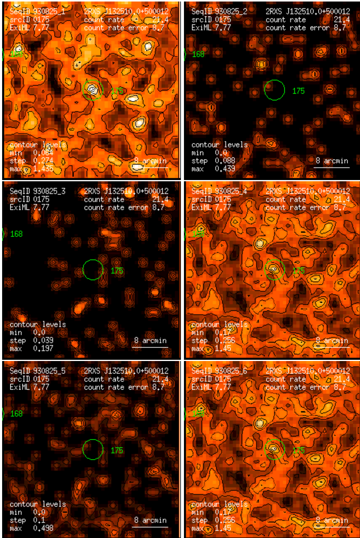
Figure 175: RASS 930825: detection 0175: band rate images, Gaussian filter: (1) PSPC channels 11 – 41, (2) 52 – 90, (3) 91 – 201, (4) 11 – 235, (5) 52 – 201, (6) 11 – 201. Broad band rates in counts/ks. Band rate contour levels in counts/ks/arcmin 2 .
