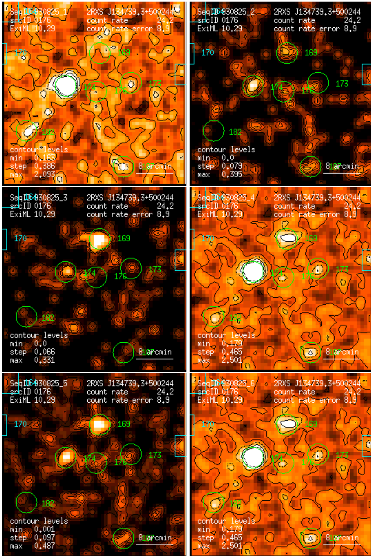
Figure 176: RASS 930825: detection 0176: band rate images, Gaussian filter: (1) PSPC channels 11 – 41, (2) 52 – 90, (3) 91 – 201, (4) 11 – 235, (5) 52 – 201, (6) 11 – 201. Broad band rates in counts/ks. Band rate contour levels in counts/ks/arcmin 2 .
