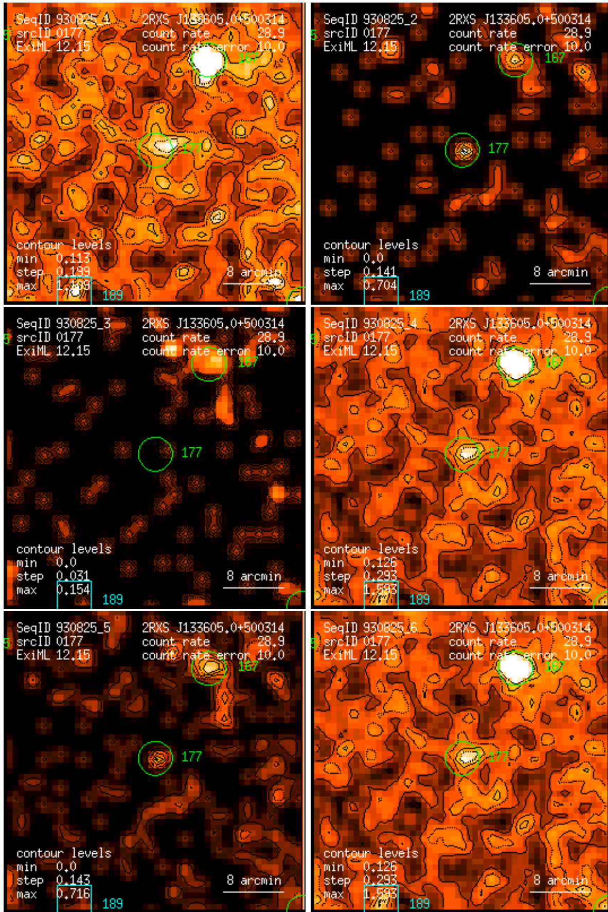
Figure 177: RASS 930825: detection 0177: band rate images, Gaussian filter: (1) PSPC channels 11 – 41, (2) 52 – 90, (3) 91 – 201, (4) 11 – 235, (5) 52 – 201, (6) 11 – 201. Broad band rates in counts/ks. Band rate contour levels in counts/ks/arcmin 2 .
