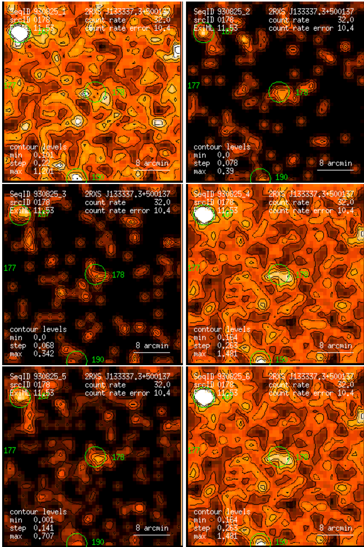
Figure 178: RASS 930825: detection 0178: band rate images, Gaussian filter: (1) PSPC channels 11 – 41, (2) 52 – 90, (3) 91 – 201, (4) 11 – 235, (5) 52 – 201, (6) 11 – 201. Broad band rates in counts/ks. Band rate contour levels in counts/ks/arcmin 2 .
