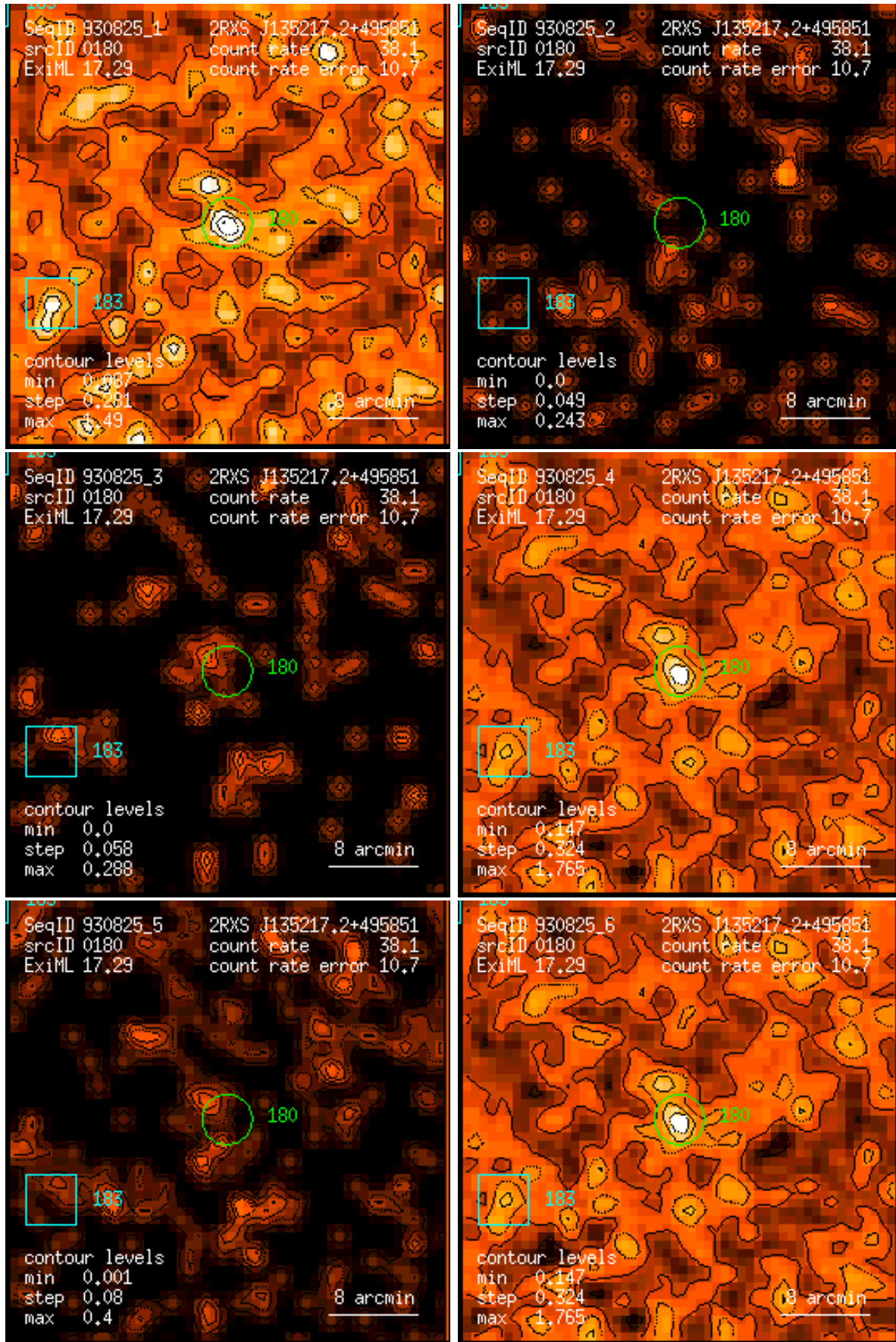
Figure 180: RASS 930825: detection 0180: band rate images, Gaussian filter: (1) PSPC channels 11 – 41, (2) 52 – 90, (3) 91 – 201, (4) 11 – 235, (5) 52 – 201, (6) 11 – 201. Broad band rates in counts/ks. Band rate contour levels in counts/ks/arcmin 2 .
