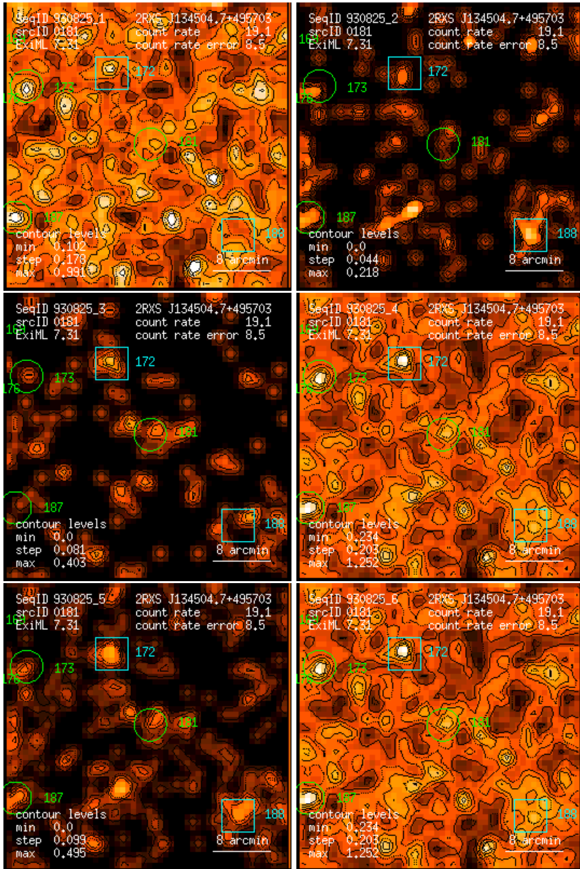
Figure 181: RASS 930825: detection 0181: band rate images, Gaussian filter: (1) PSPC channels 11 – 41, (2) 52 – 90, (3) 91 – 201, (4) 11 – 235, (5) 52 – 201, (6) 11 – 201. Broad band rates in counts/ks. Band rate contour levels in counts/ks/arcmin 2 .
