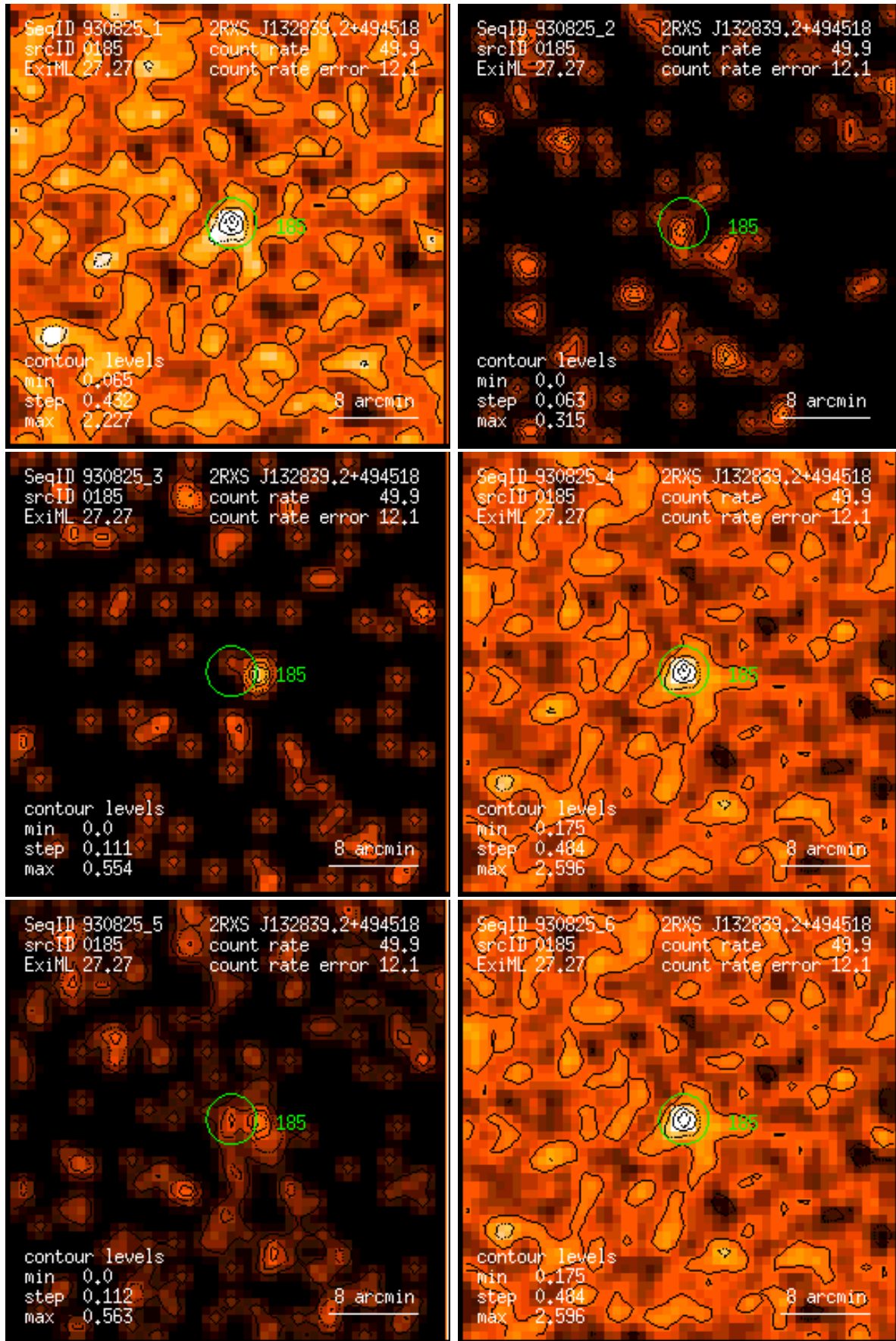
Figure 185: RASS 930825: detection 0185: band rate images, Gaussian filter: (1) PSPC channels 11 – 41, (2) 52 – 90, (3) 91 – 201, (4) 11 – 235, (5) 52 – 201, (6) 11 – 201. Broad band rates in counts/ks. Band rate contour levels in counts/ks/arcmin 2 .
