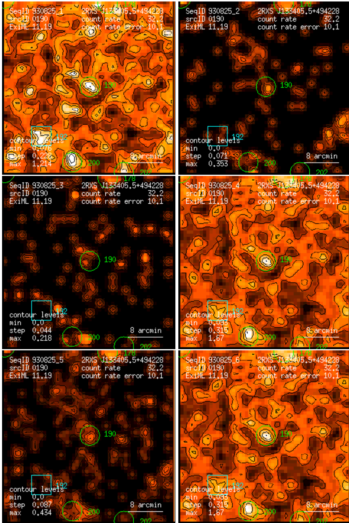
Figure 190: RASS 930825: detection 0190: band rate images, Gaussian filter: (1) PSPC channels 11 – 41, (2) 52 – 90, (3) 91 – 201, (4) 11 – 235, (5) 52 – 201, (6) 11 – 201. Broad band rates in counts/ks. Band rate contour levels in counts/ks/arcmin 2 .
