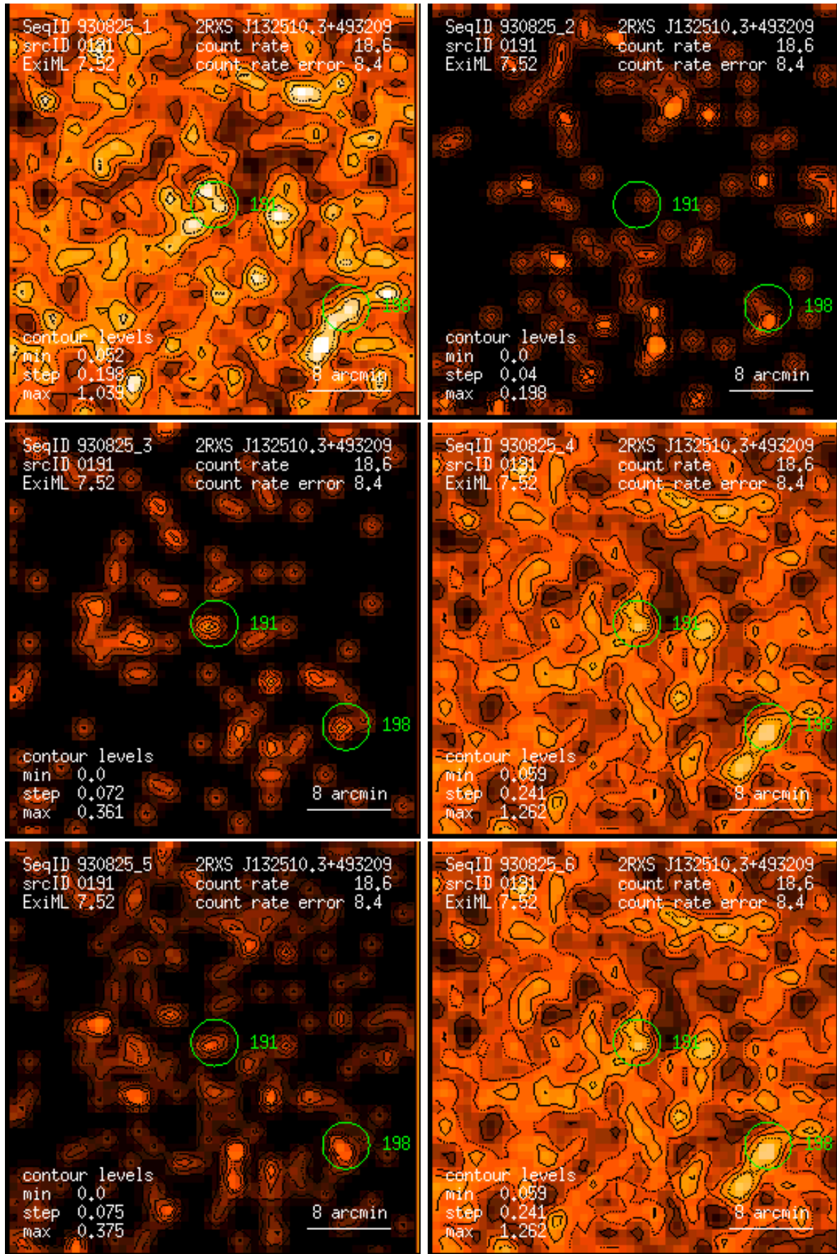
Figure 191: RASS 930825: detection 0191: band rate images, Gaussian filter: (1) PSPC channels 11 – 41, (2) 52 – 90, (3) 91 – 201, (4) 11 – 235, (5) 52 – 201, (6) 11 – 201. Broad band rates in counts/ks. Band rate contour levels in counts/ks/arcmin 2 .
