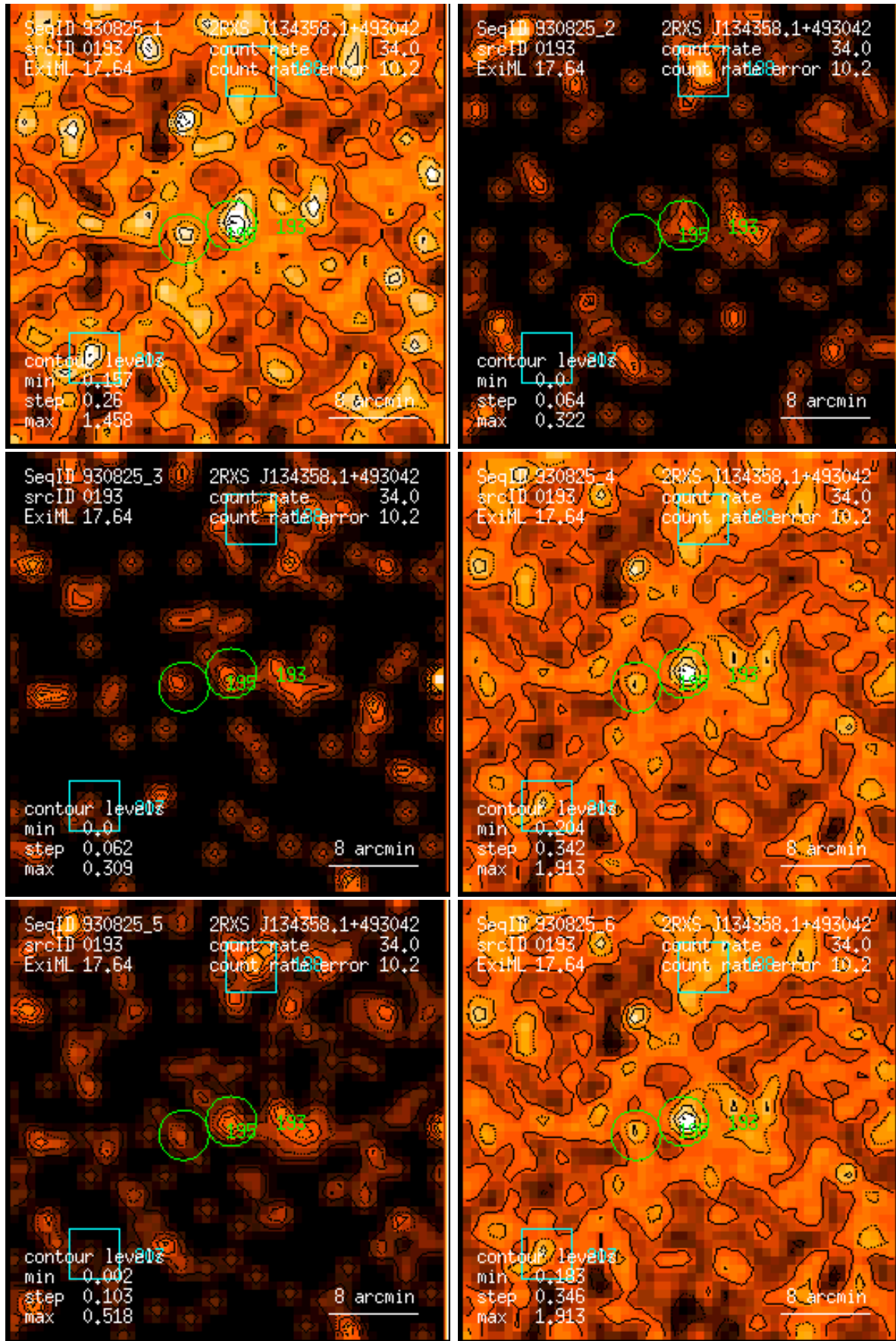
Figure 193: RASS 930825: detection 0193: band rate images, Gaussian filter: (1) PSPC channels 11 – 41, (2) 52 – 90, (3) 91 – 201, (4) 11 – 235, (5) 52 – 201, (6) 11 – 201. Broad band rates in counts/ks. Band rate contour levels in counts/ks/arcmin 2 .
