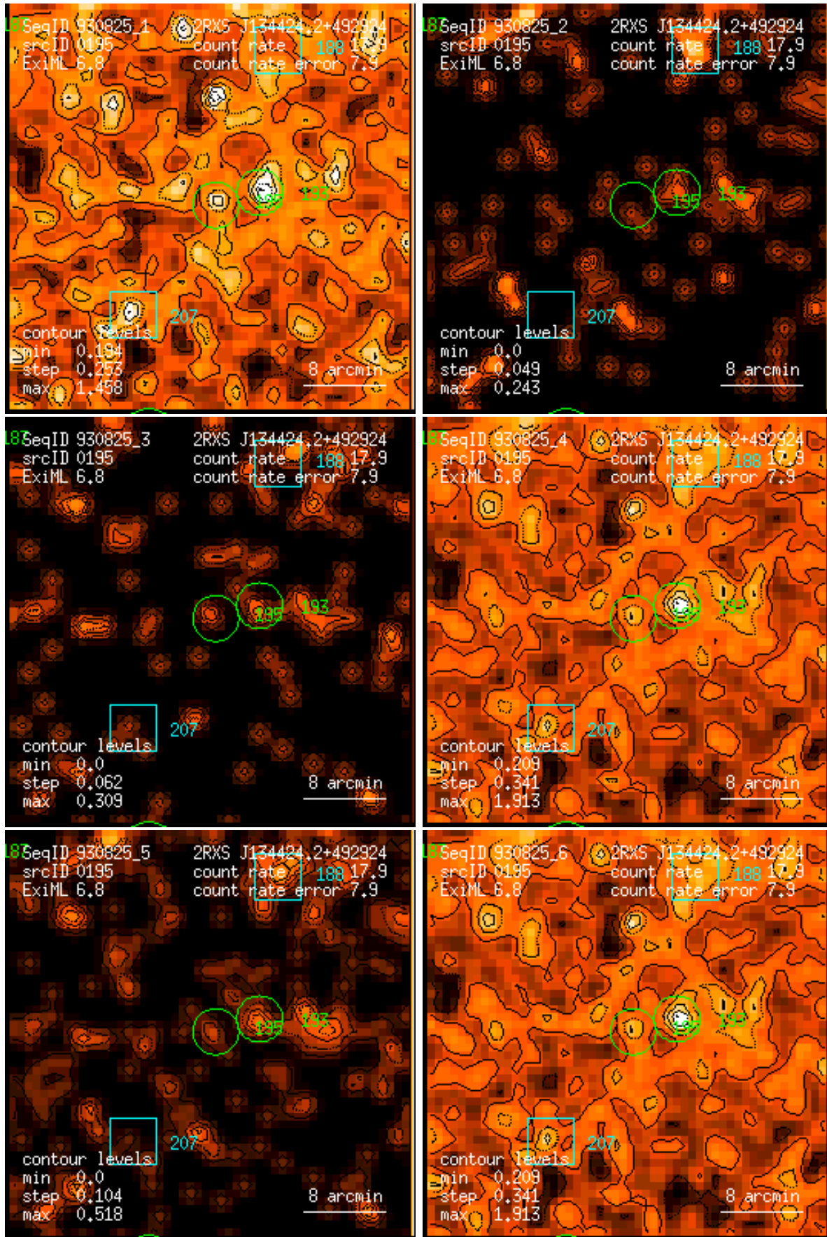
Figure 195: RASS 930825: detection 0195: band rate images, Gaussian filter: (1) PSPPC channels 11 – 41, (2) 52 – 90, (3) 91 – 201, (4) 11 – 235, (5) 52 – 201, (6) 11 – 201. Broad band rates in counts/ks. Band rate contour levels in counts/ks/arcmin 2 .
