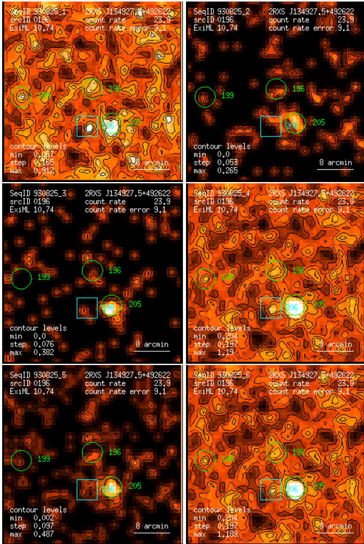
Figure 196: RASS 930825: detection 0196: band rate images, Gaussian filter: (1) PSPC channels 11 – 41, (2) 52 – 90, (3) 91 – 201, (4) 11 – 235, (5) 52 – 201, (6) 11 – 201. Broad band rates in counts/ks. Band rate contour levels in counts/ks/arcmin 2 .
