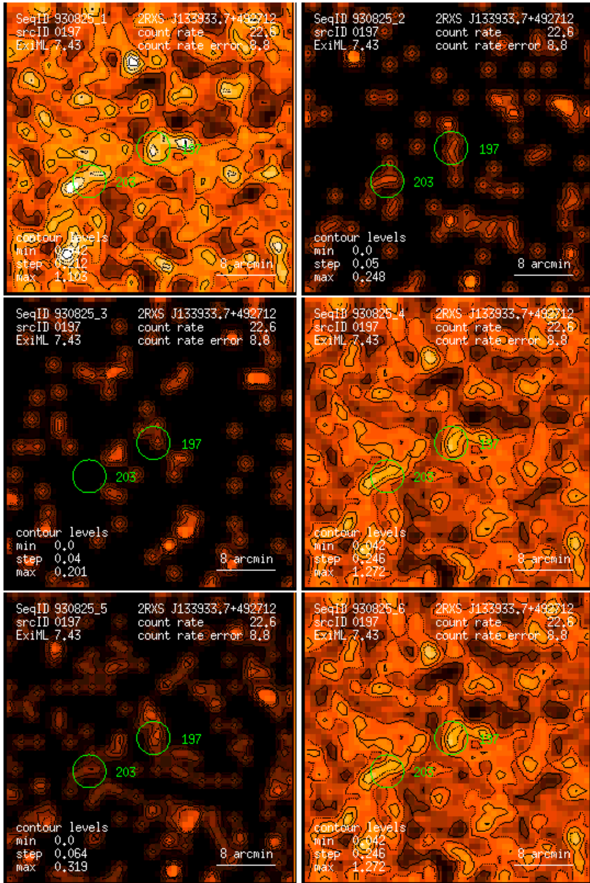
Figure 197: RASS 930825: detection 0197: band rate images, Gaussian filter: (1) PSPC channels 11 – 41, (2) 52 – 90, (3) 91 – 201, (4) 11 – 235, (5) 52 – 201, (6) 11 – 201. Broad band rates in counts/ks. Band rate contour levels in counts/ks/arcmin 2 .
