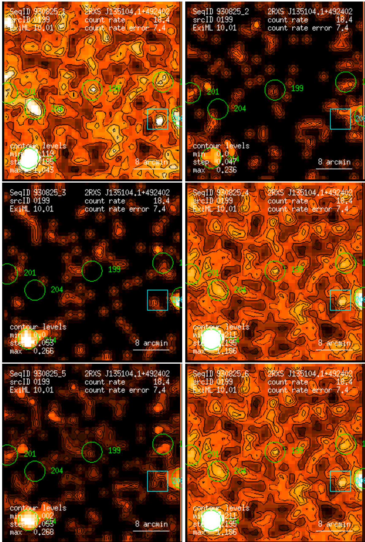
Figure 199: RASS 930825: detection 0199: band rate images, Gaussian filter: (1) PSPC channels 11 – 41, (2) 52 – 90, (3) 91 – 201, (4) 11 – 235, (5) 52 – 201, (6) 11 – 201. Broad band rates in counts/ks. Band rate contour levels in counts/ks/arcmin 2 .
