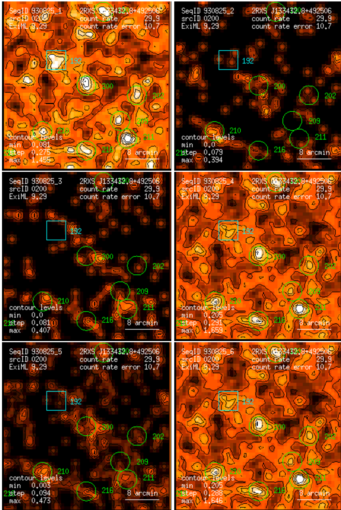
Figure 200: RASS 930825: detection 0200: band rate images, Gaussian filter: (1) PSPC channels 11 – 41, (2) 52 – 90, (3) 91 – 201, (4) 11 – 235, (5) 52 – 201, (6) 11 – 201. Broad band rates in counts/ks. Band rate contour levels in counts/ks/arcmin 2 .
