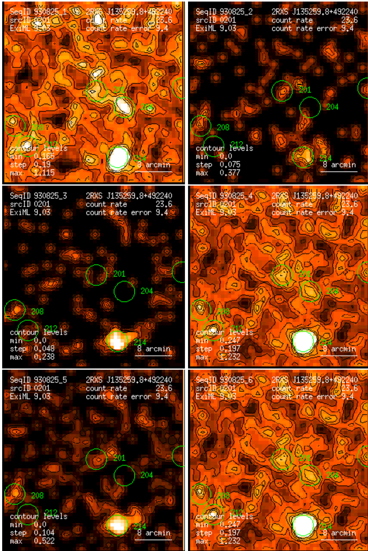
Figure 201: RASS 930825: detection 0201: band rate images, Gaussian filter: (1) PSPC channels 11 – 41, (2) 52 – 90, (3) 91 – 201, (4) 11 – 235, (5) 52 – 201, (6) 11 – 201. Broad band rates in counts/ks. Band rate contour levels in counts/ks/arcmin 2 .
