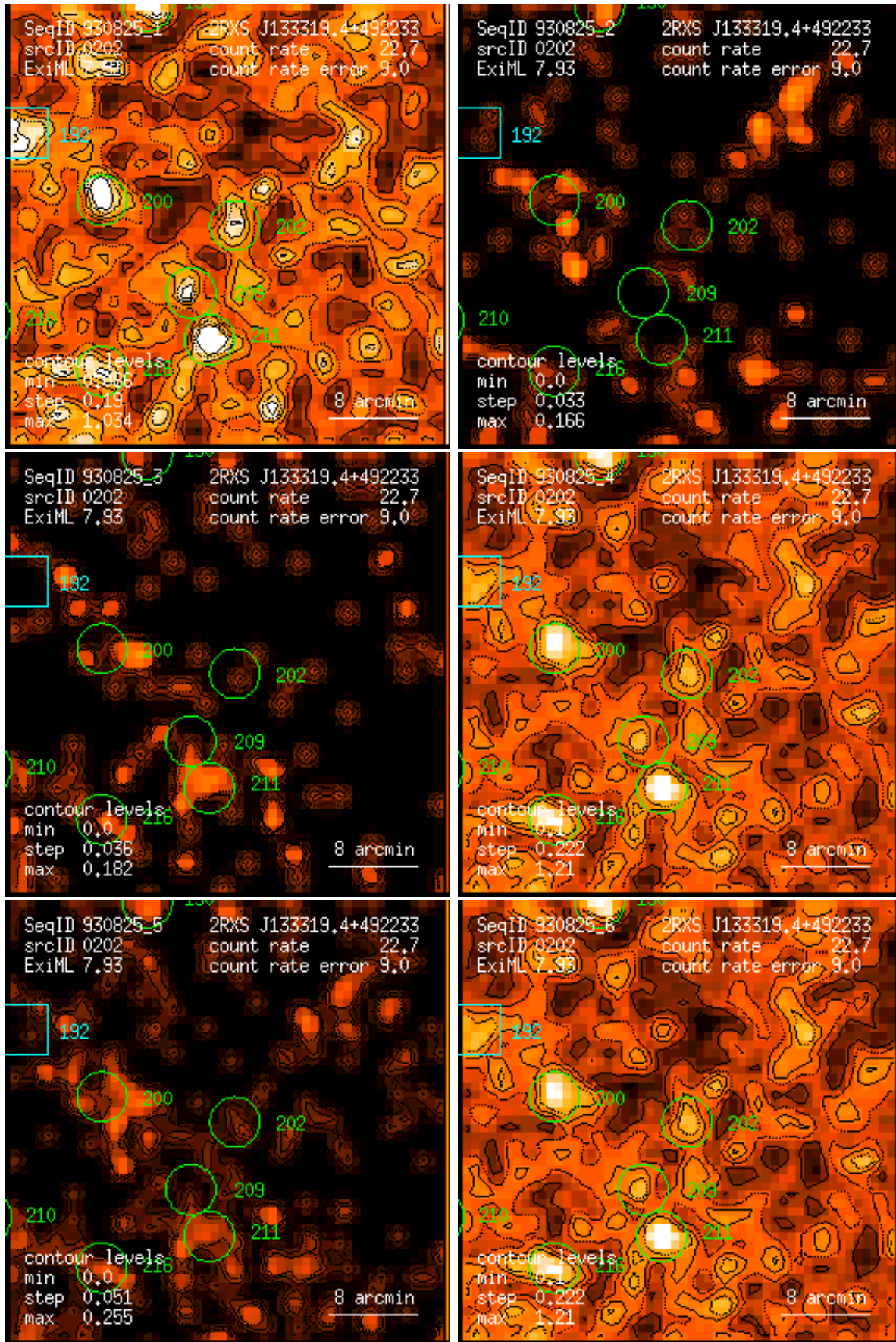
Figure 202: RASS 930825: detection 0202: band rate images, Gaussian filter: (1) PSPC channels 11 – 41, (2) 52 – 90, (3) 91 – 201, (4) 11 – 235, (5) 52 – 201, (6) 11 – 201. Broad band rates in counts/ks. Band rate contour levels in counts/ks/arcmin 2 .
