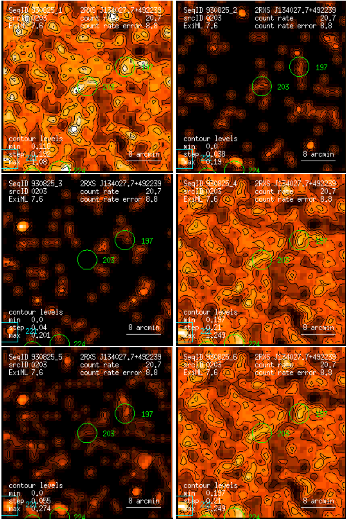
Figure 203: RASS 930825: detection 0203: band rate images, Gaussian filter: (1) PSPC channels 11 – 41, (2) 52 – 90, (3) 91 – 201, (4) 11 – 235, (5) 52 – 201, (6) 11 – 201. Broad band rates in counts/ks. Band rate contour levels in counts/ks/arcmin 2 .
