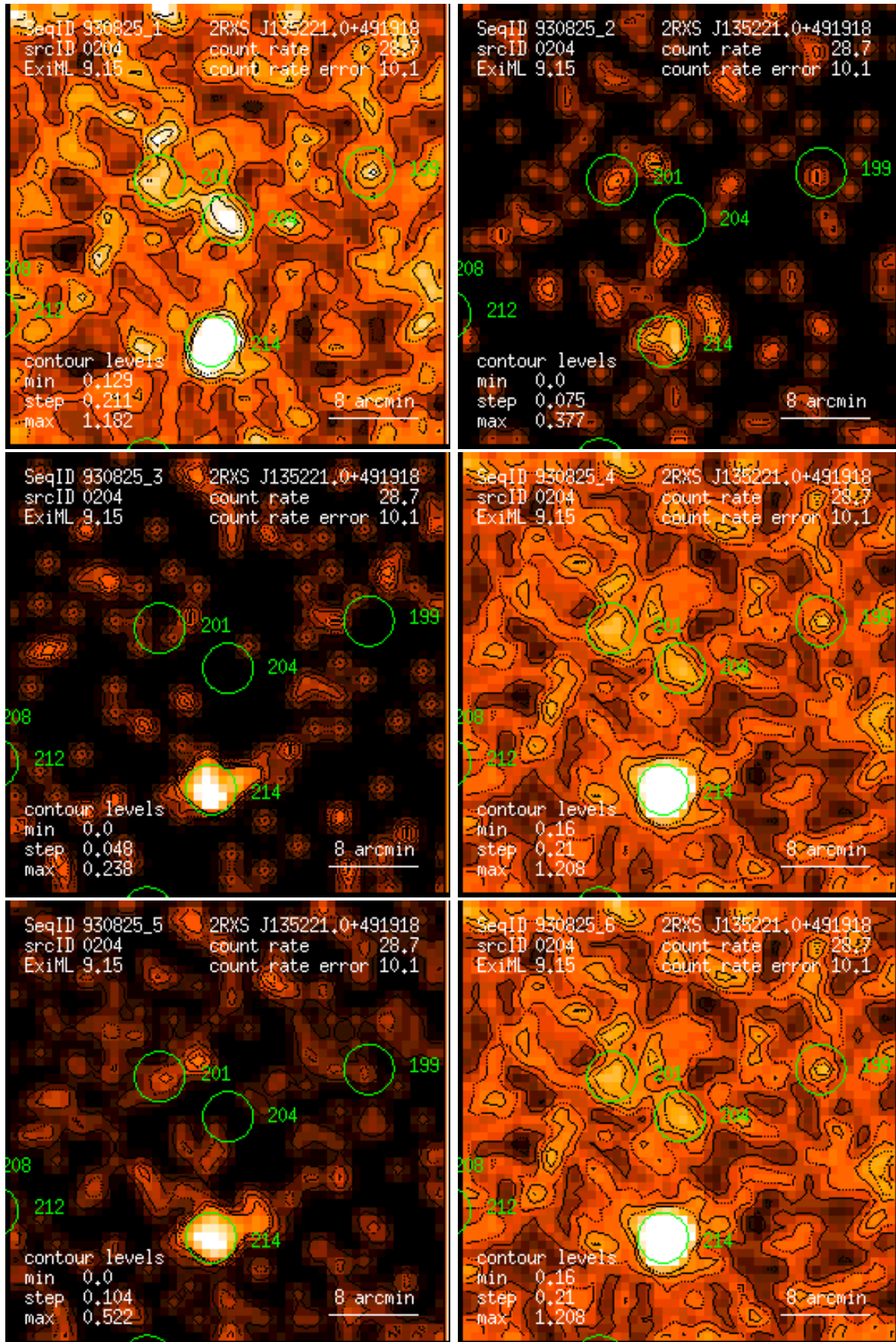
Figure 204: RASS 930825: detection 0204: band rate images, Gaussian filter: (1) PSPC channels 11 – 41, (2) 52 – 90, (3) 91 – 201, (4) 11 – 235, (5) 52 – 201, (6) 11 – 201. Broad band rates in counts/ks. Band rate contour levels in counts/ks/arcmin 2 .
