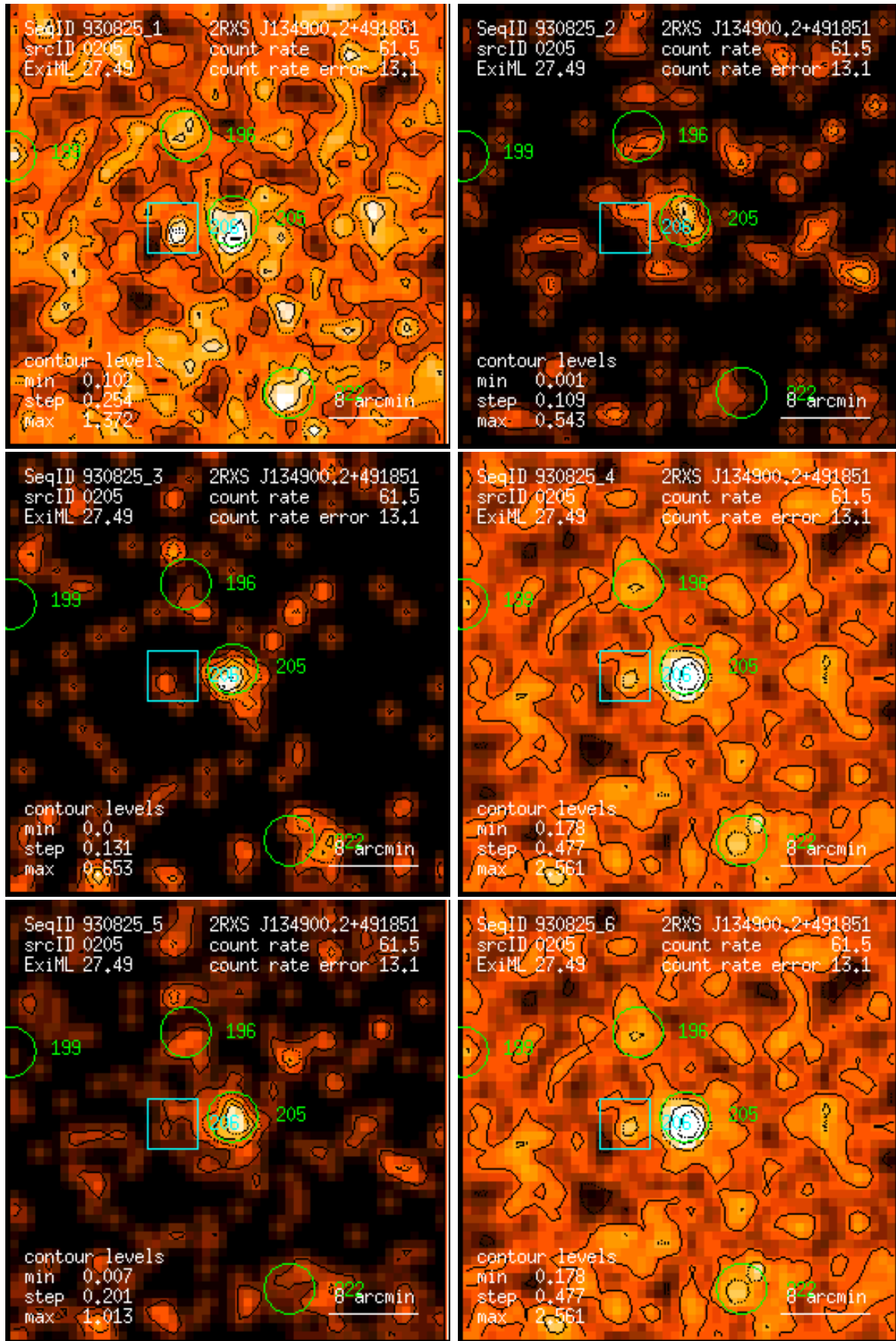
Figure 205: RASS 930825: detection 0205: band rate images, Gaussian filter: (1) PSPC channels 11 – 41, (2) 52 – 90, (3) 91 – 201, (4) 11 – 235, (5) 52 – 201, (6) 11 – 201. Broad band rates in counts/ks. Band rate contour levels in counts/ks/arcmin 2 .
