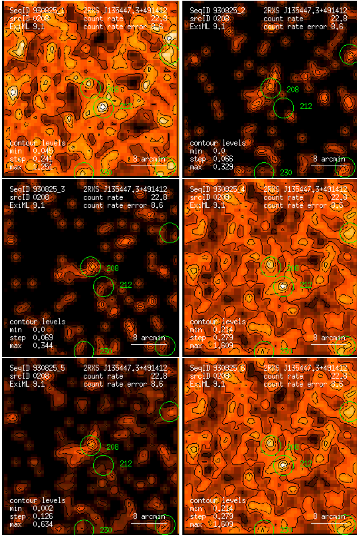
Figure 208: RASS 930825: detection 0208: band rate images, Gaussian filter: (1) PSPC channels 11 – 41, (2) 52 – 90, (3) 91 – 201, (4) 11 – 235, (5) 52 – 201, (6) 11 – 201. Broad band rates in counts/ks. Band rate contour levels in counts/ks/arcmin 2 .
