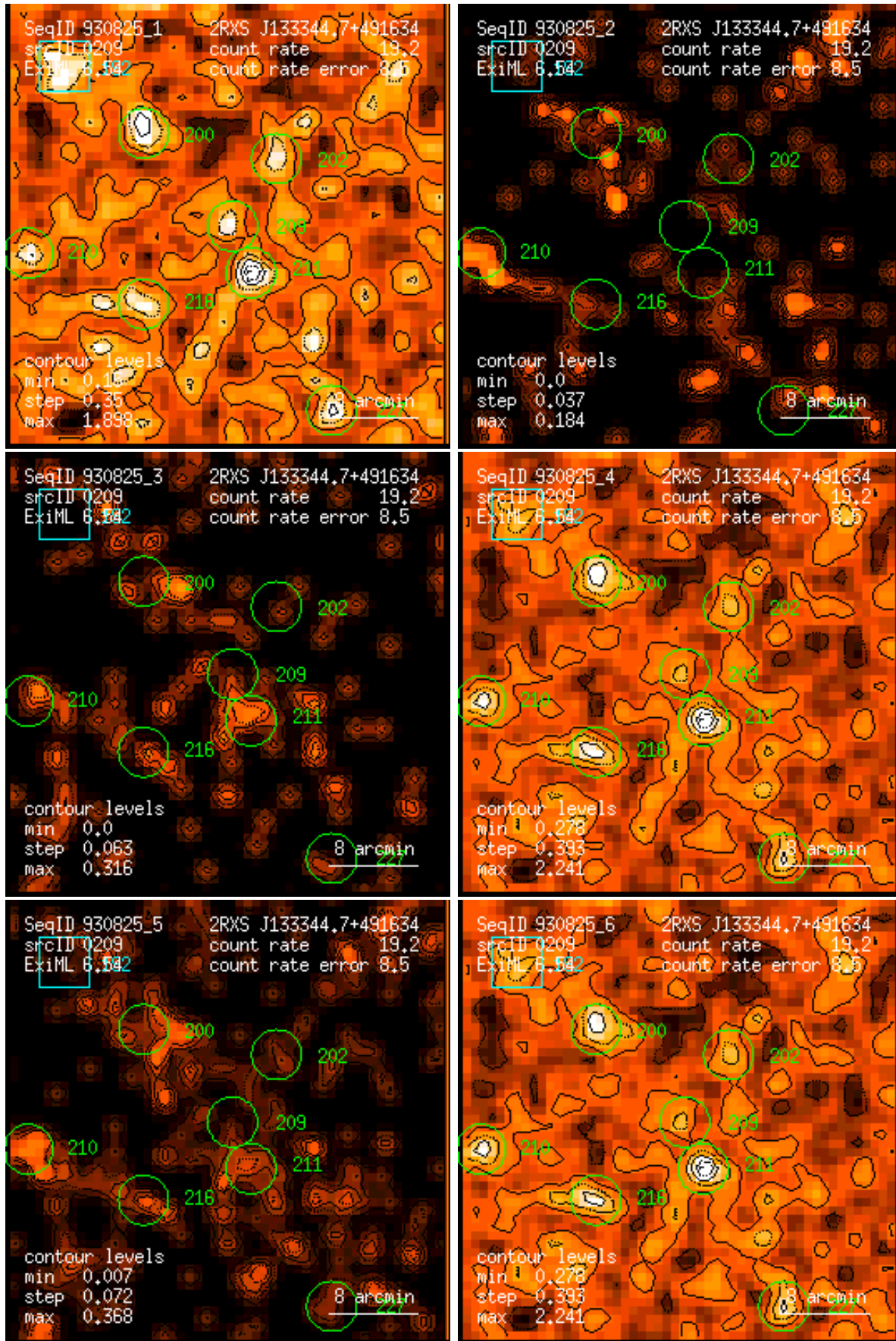
Figure 209: RASS 930825: detection 0209: band rate images, Gaussian filter: (1) PSPC channels 11 – 41, (2) 52 – 90, (3) 91 – 201, (4) 11 – 235, (5) 52 – 201, (6) 11 – 201. Broad band rates in counts/ks. Band rate contour levels in counts/ks/arcmin 2 .
