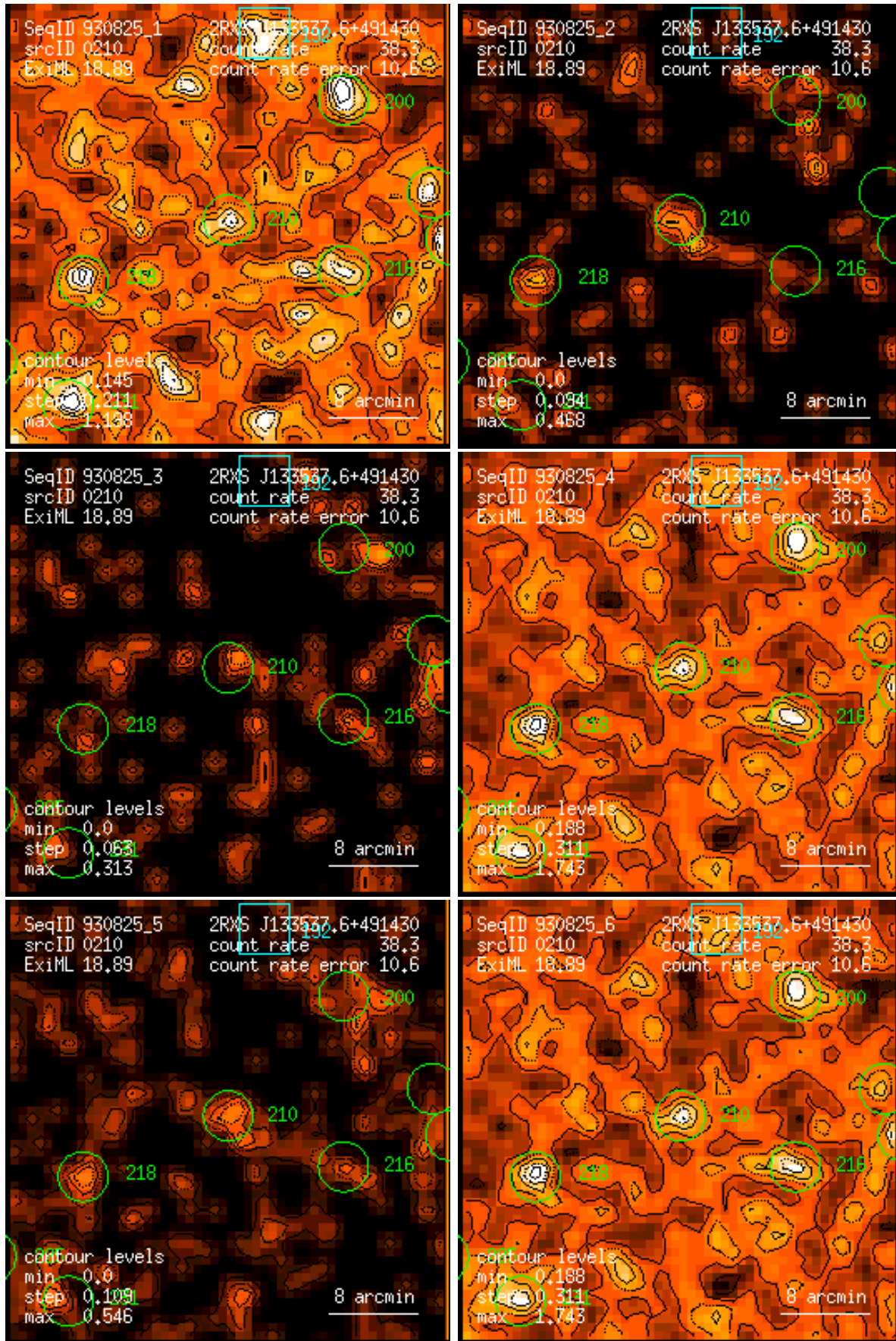
Figure 210: RASS 930825: detection 0210: band rate images, Gaussian filter: (1) PSPC channels 11 – 41, (2) 52 – 90, (3) 91 – 201, (4) 11 – 235, (5) 52 – 201, (6) 11 – 201. Broad band rates in counts/ks. Band rate contour levels in counts/ks/arcmin 2 .
