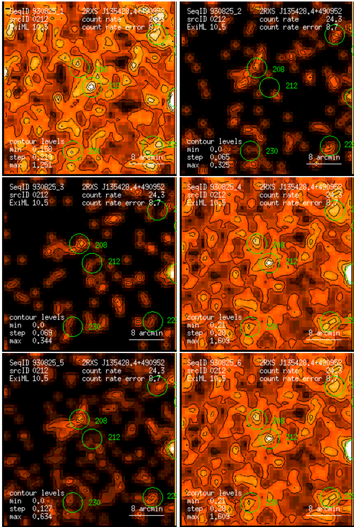
Figure 212: RASS 930825: detection 0212: band rate images, Gaussian filter: (1) PSPC channels 11 – 41, (2) 52 – 90, (3) 91 – 201, (4) 11 – 235, (5) 52 – 201, (6) 11 – 201. Broad band rates in counts/ks. Band rate contour levels in counts/ks/arcmin 2 .
