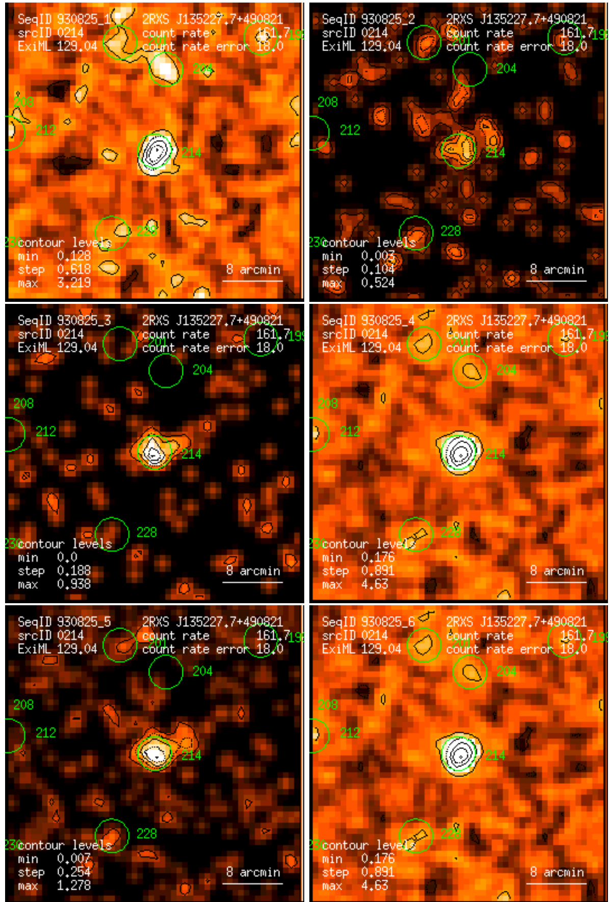
Figure 214: RASS 930825: detection 0214: band rate images, Gaussian filter: (1) PSPC channels 11 – 41, (2) 52 – 90, (3) 91 – 201, (4) 11 – 235, (5) 52 – 201, (6) 11 – 201. Broad band rates in counts/ks. Band rate contour levels in counts/ks/arcmin 2 .
