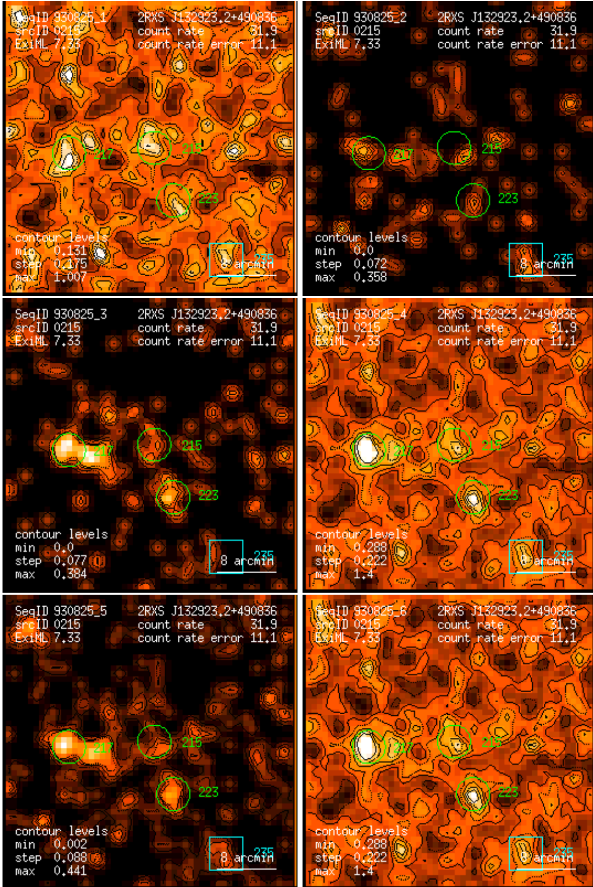
Figure 215: RASS 930825: detection 0215: band rate images, Gaussian filter: (1) PSPC channels 11 – 41, (2) 52 – 90, (3) 91 – 201, (4) 11 – 235, (5) 52 – 201, (6) 11 – 201. Broad band rates in counts/ks. Band rate contour levels in counts/ks/arcmin 2 .
