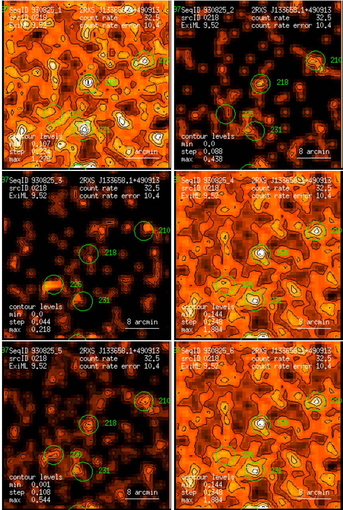
Figure 218: RASS 930825: detection 0218: band rate images, Gaussian filter: (1) PSPC channels 11 – 41, (2) 52 – 90, (3) 91 – 201, (4) 11 – 235, (5) 52 – 201, (6) 11 – 201. Broad band rates in counts/ks. Band rate contour levels in counts/ks/arcmin 2 .
