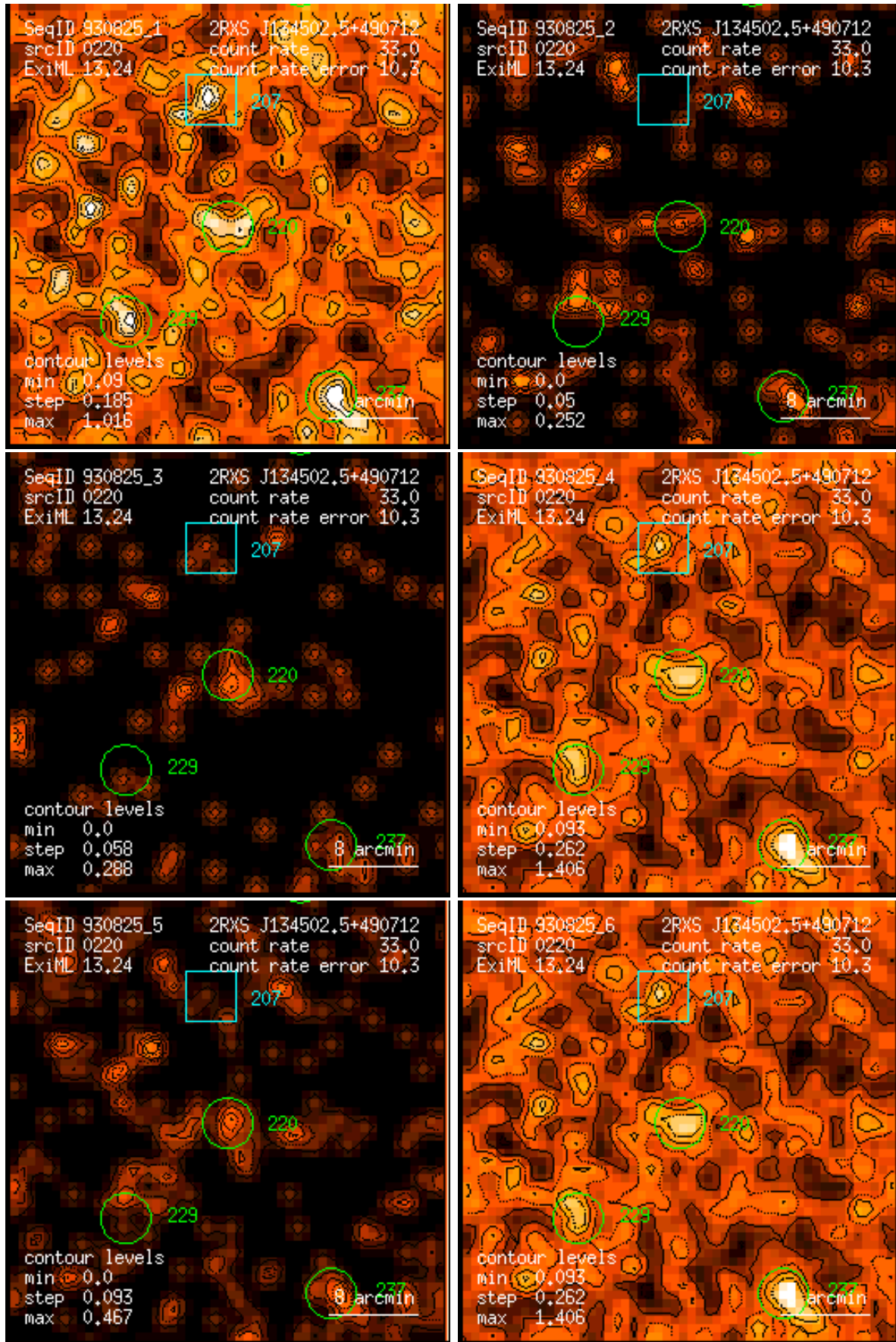
Figure 220: RASS 930825: detection 0220: band rate images, Gaussian filter: (1) PSPC channels 11 – 41, (2) 52 – 90, (3) 91 – 201, (4) 11 – 235, (5) 52 – 201, (6) 11 – 201. Broad band rates in counts/ks. Band rate contour levels in counts/ks/arcmin 2 .
