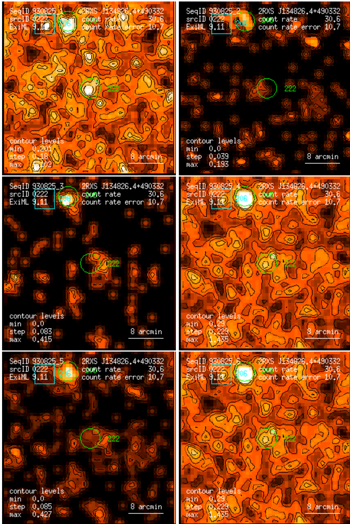
Figure 222: RASS 930825: detection 0222: band rate images, Gaussian filter: (1) PSPC channels 11 – 41, (2) 52 – 90, (3) 91 – 201, (4) 11 – 235, (5) 52 – 201, (6) 11 – 201. Broad band rates in counts/ks. Band rate contour levels in counts/ks/arcmin 2 .
