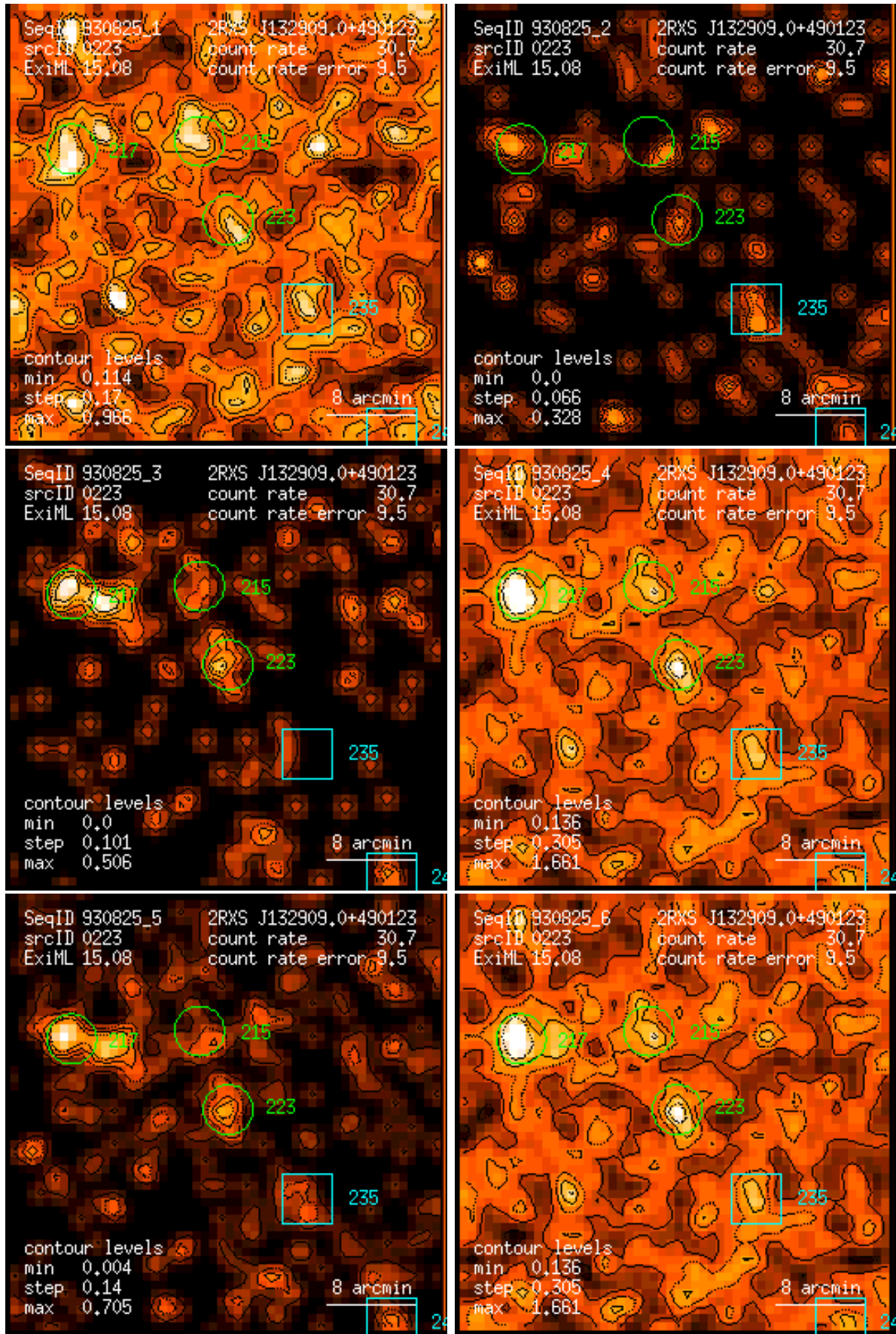
Figure 223: RASS 930825: detection 0223: band rate images, Gaussian filter: (1) PSPC channels 11 – 41, (2) 52 – 90, (3) 91 – 201, (4) 11 – 235, (5) 52 – 201, (6) 11 – 201. Broad band rates in counts/ks. Band rate contour levels in counts/ks/arcmin 2 .
