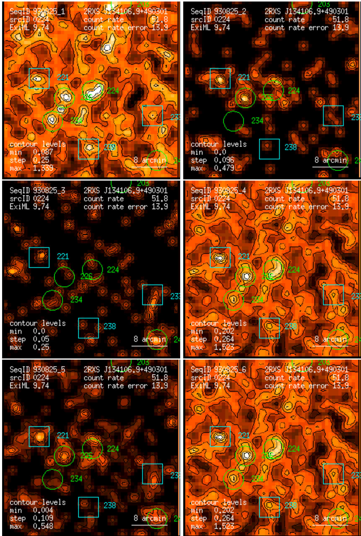
Figure 224: RASS 930825: detection 0224: band rate images, Gaussian filter: (1) PSPC channels 11 – 41, (2) 52 – 90, (3) 91 – 201, (4) 11 – 235, (5) 52 – 201, (6) 11 – 201. Broad band rates in counts/ks. Band rate contour levels in counts/ks/arcmin 2 .
