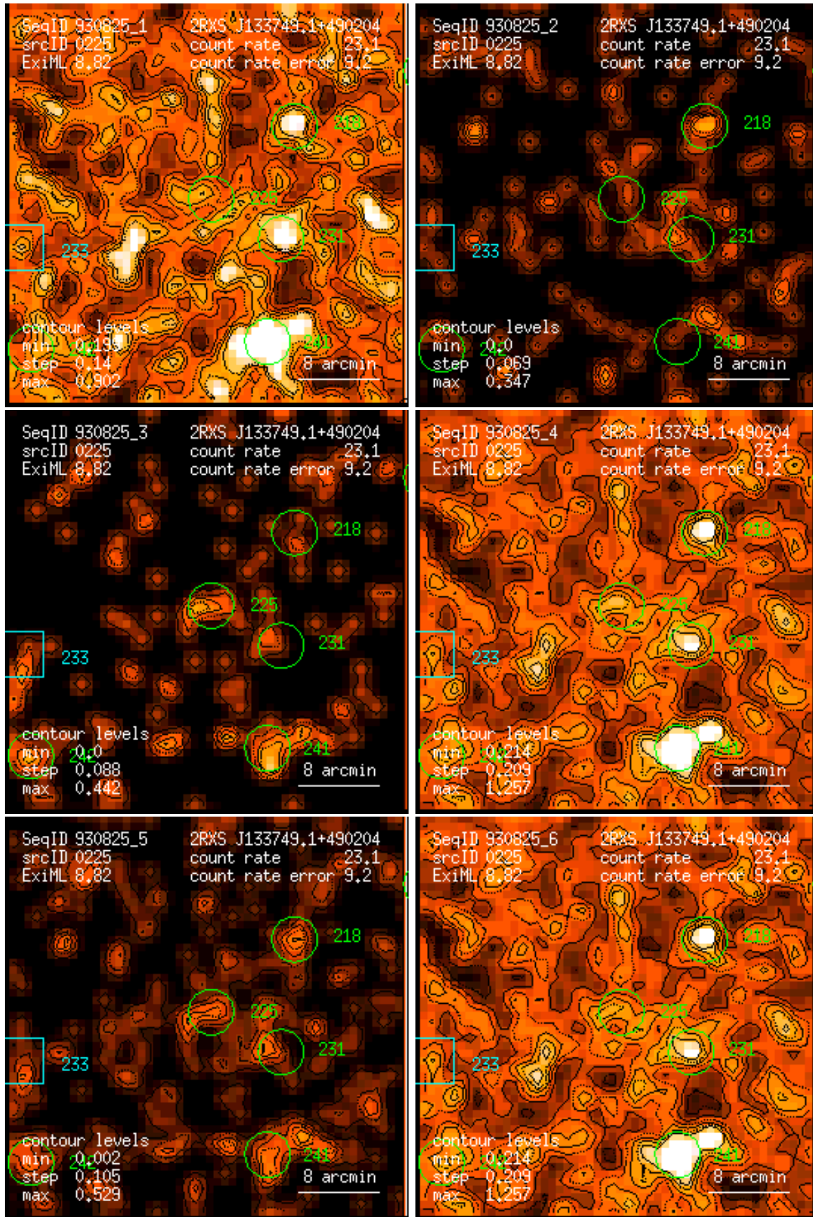
Figure 225: RASS 930825: detection 0225: band rate images, Gaussian filter: (1) PSPC channels 11 – 41, (2) 52 – 90, (3) 91 – 201, (4) 11 – 235, (5) 52 – 201, (6) 11 – 201. Broad band rates in counts/ks. Band rate contour levels in counts/ks/arcmin 2 .
