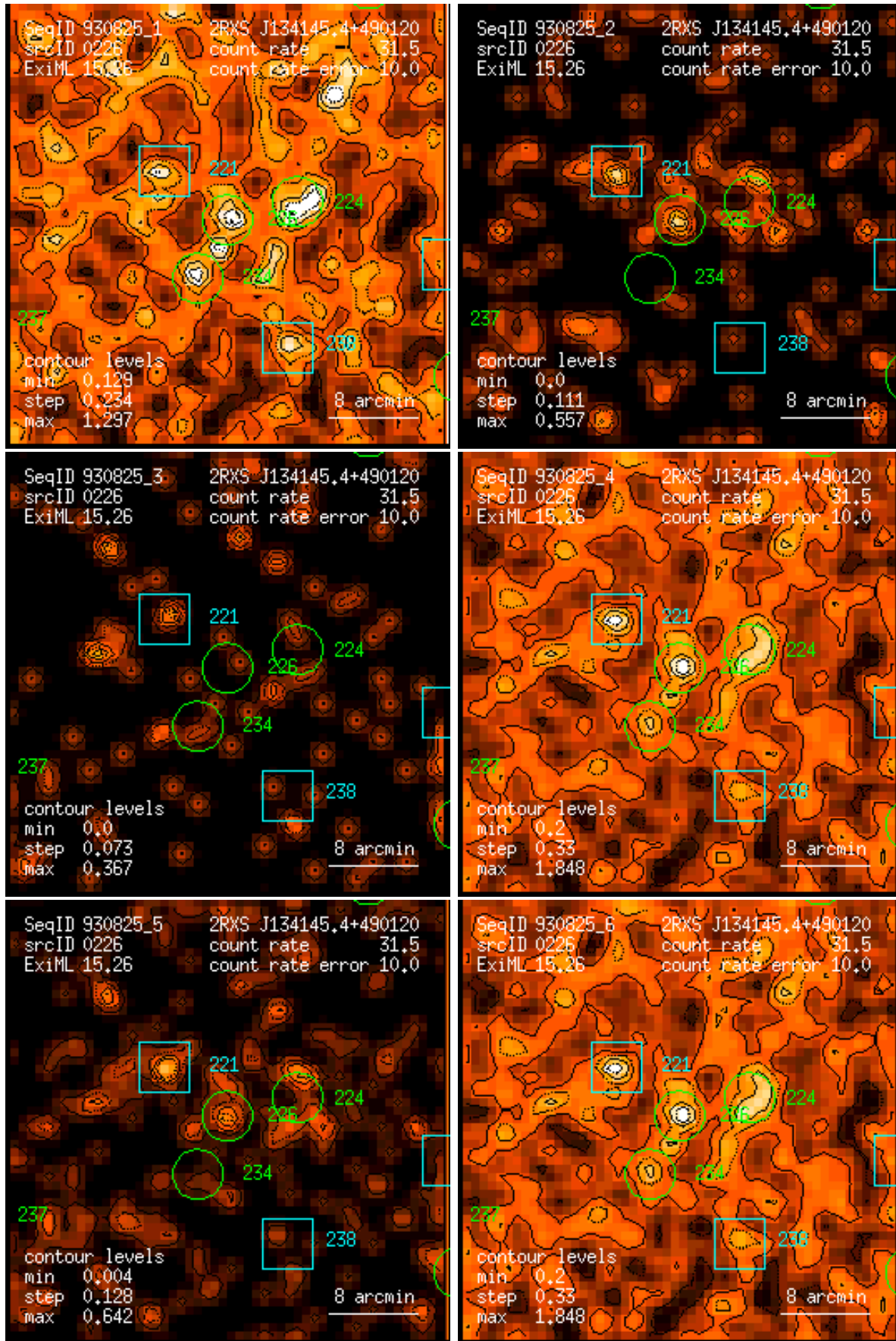
Figure 226: RASS 930825: detection 0226: band rate images, Gaussian filter: (1) PSPC channels 11 – 41, (2) 52 – 90, (3) 91 – 201, (4) 11 – 235, (5) 52 – 201, (6) 11 – 201. Broad band rates in counts/ks. Band rate contour levels in counts/ks/arcmin 2 .
