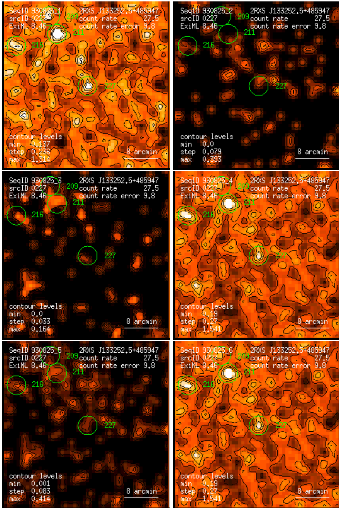
Figure 227: RASS 930825: detection 0227: band rate images, Gaussian filter: (1) PSPC channels 11 – 41, (2) 52 – 90, (3) 91 – 201, (4) 11 – 235, (5) 52 – 201, (6) 11 – 201. Broad band rates in counts/ks. Band rate contour levels in counts/ks/arcmin 2 .
