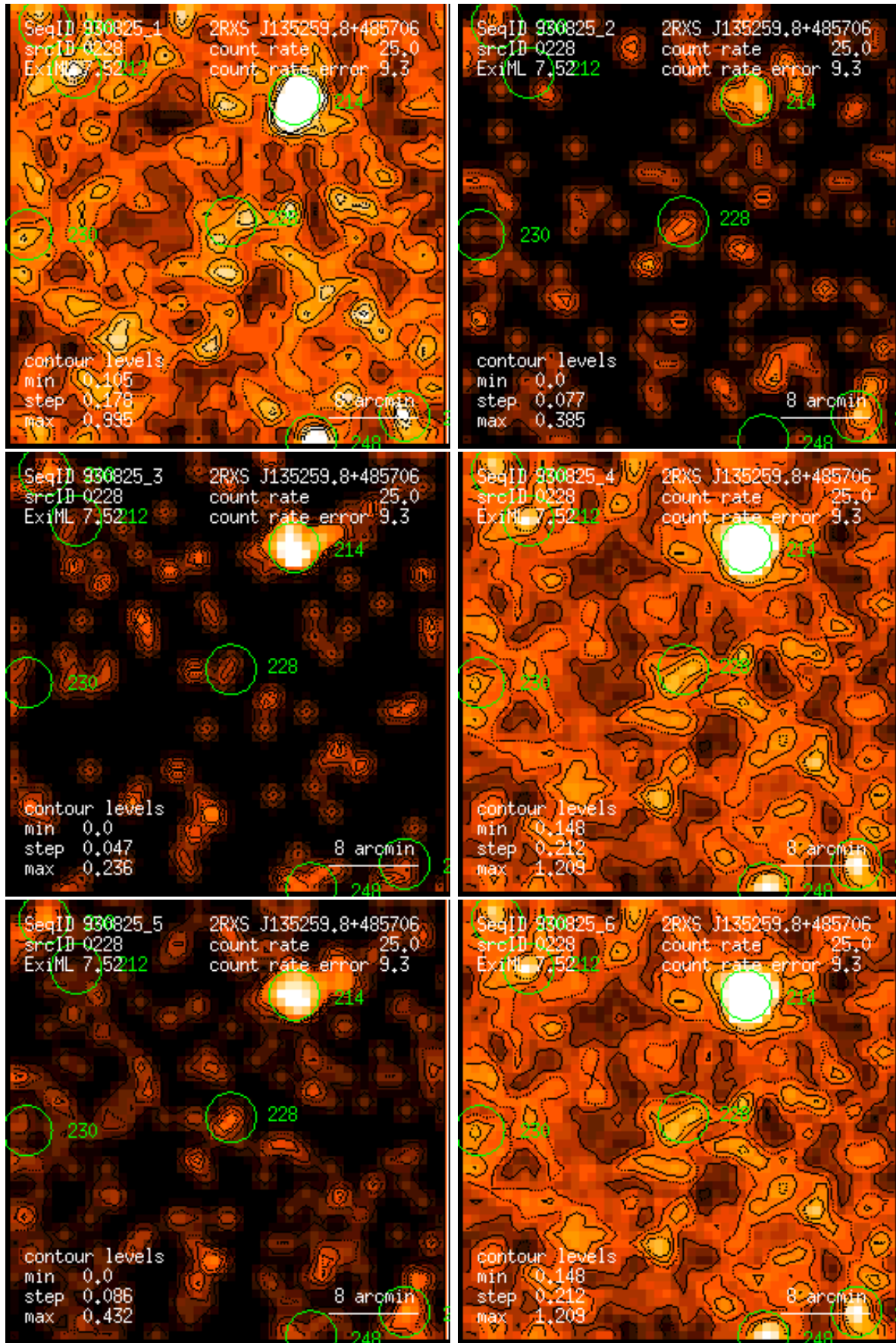
Figure 228: RASS 930825: detection 0228: band rate images, Gaussian filter: (1) PSPC channels 11 – 41, (2) 52 – 90, (3) 91 – 201, (4) 11 – 235, (5) 52 – 201, (6) 11 – 201. Broad band rates in counts/ks. Band rate contour levels in counts/ks/arcmin 2 .
