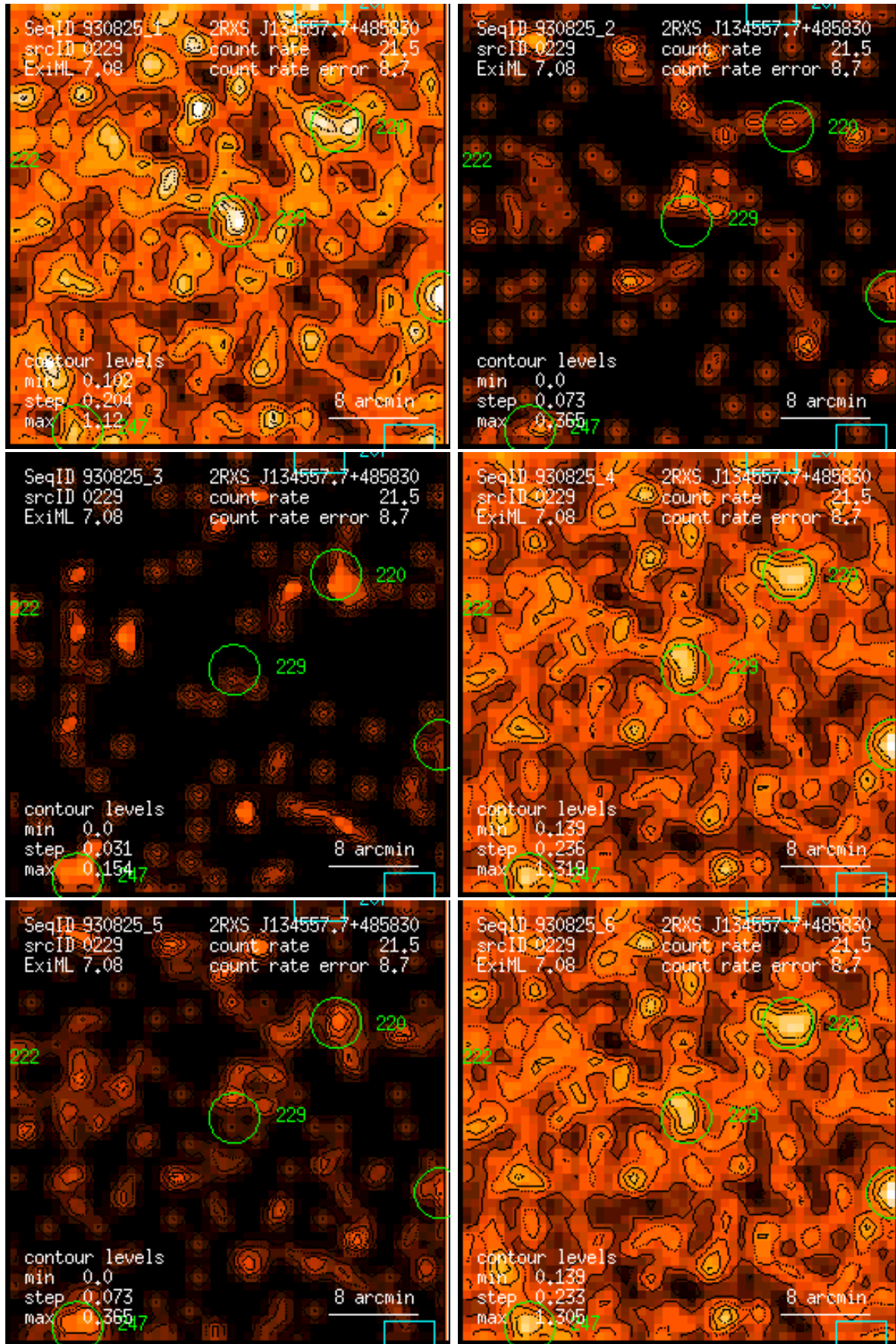
Figure 229: RASS 930825: detection 0229: band rate images, Gaussian filter: (1) PSPC channels 11 – 41, (2) 52 – 90, (3) 91 – 201, (4) 11 – 235, (5) 52 – 201, (6) 11 – 201. Broad band rates in counts/ks. Band rate contour levels in counts/ks/arcmin 2 .
