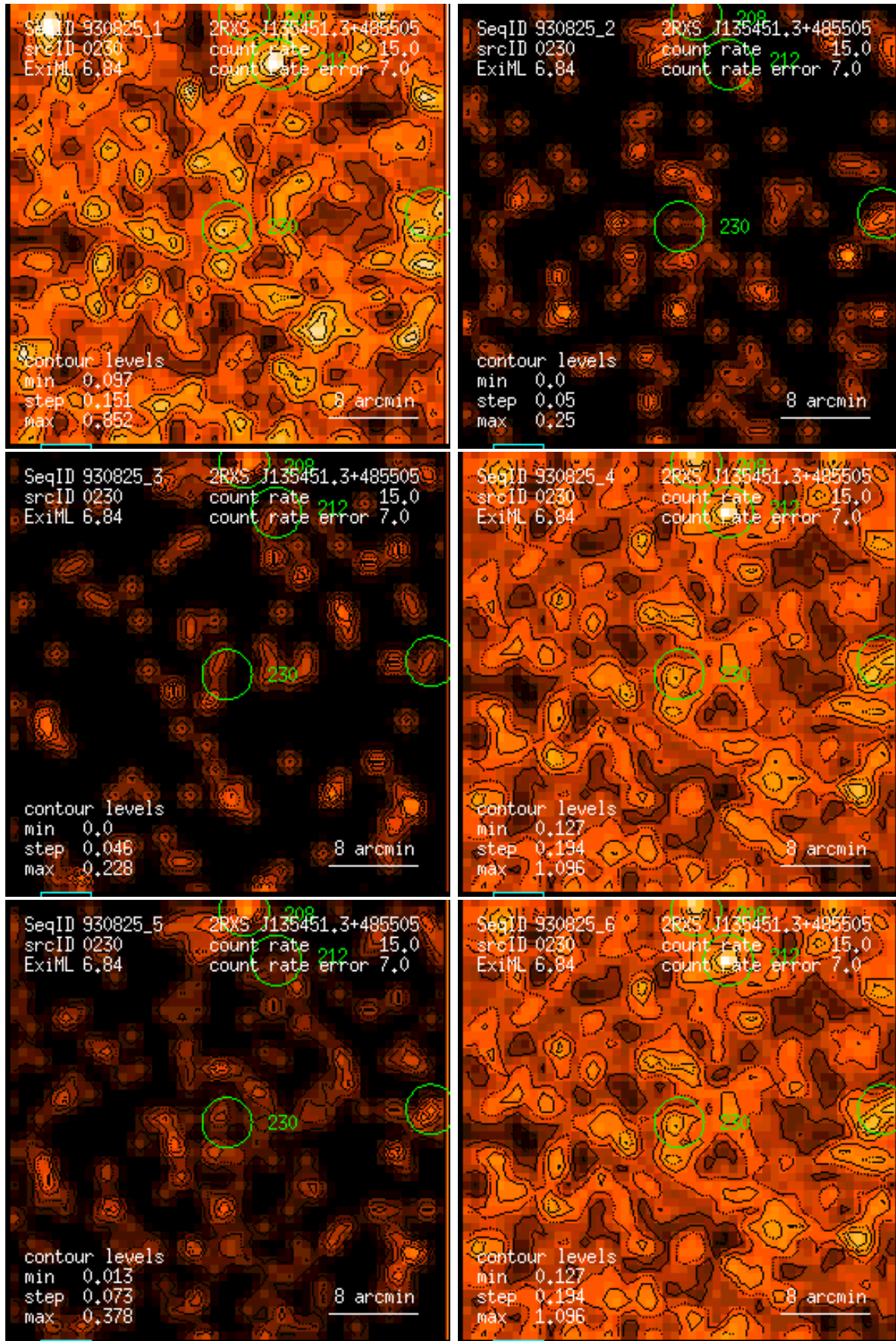
Figure 230: RASS 930825: detection 0230: band rate images, Gaussian filter: (1) PSPC channels 11 – 41, (2) 52 – 90, (3) 91 – 201, (4) 11 – 235, (5) 52 – 201, (6) 11 – 201. Broad band rates in counts/ks. Band rate contour levels in counts/ks/arcmin 2 .
