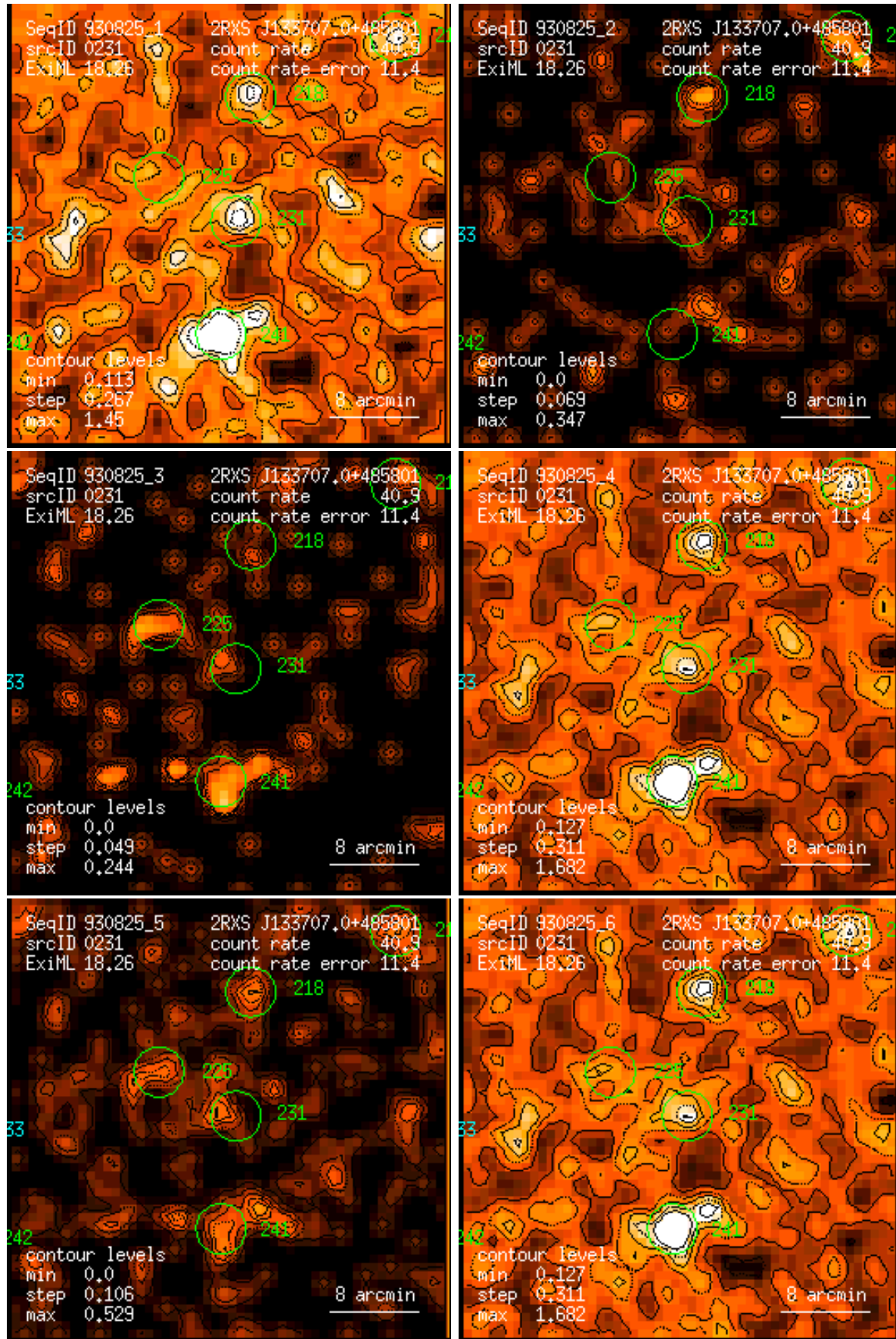
Figure 231: RASS 930825: detection 0231: band rate images, Gaussian filter: (1) PSPC channels 11 – 41, (2) 52 – 90, (3) 91 – 201, (4) 11 – 235, (5) 52 – 201, (6) 11 – 201. Broad band rates in counts/ks. Band rate contour levels in counts/ks/arcmin 2 .
