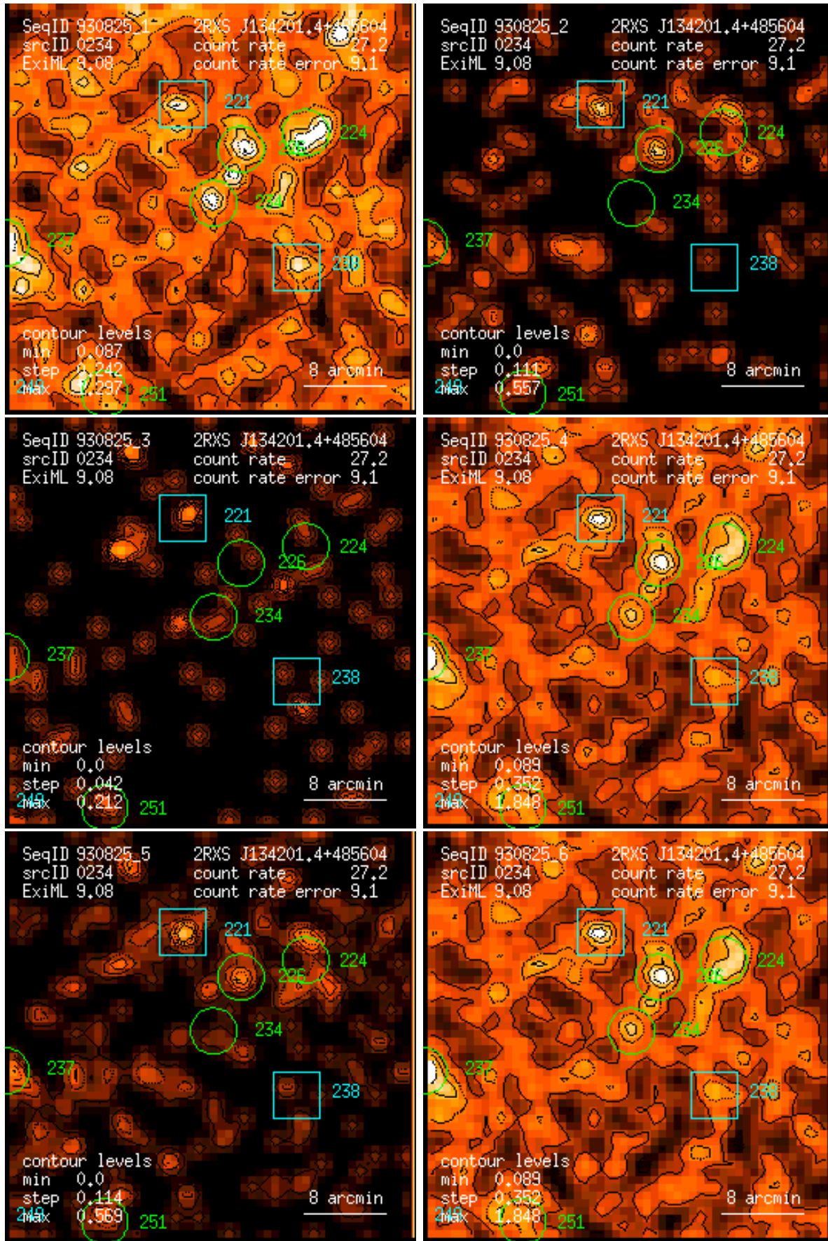
Figure 234: RASS 930825: detection 0234: band rate images, Gaussian filter: (1) PSPC channels 11 – 41, (2) 52 – 90, (3) 91 – 201, (4) 11 – 235, (5) 52 – 201, (6) 11 – 201. Broad band rates in counts/ks. Band rate contour levels in counts/ks/arcmin 2 .
