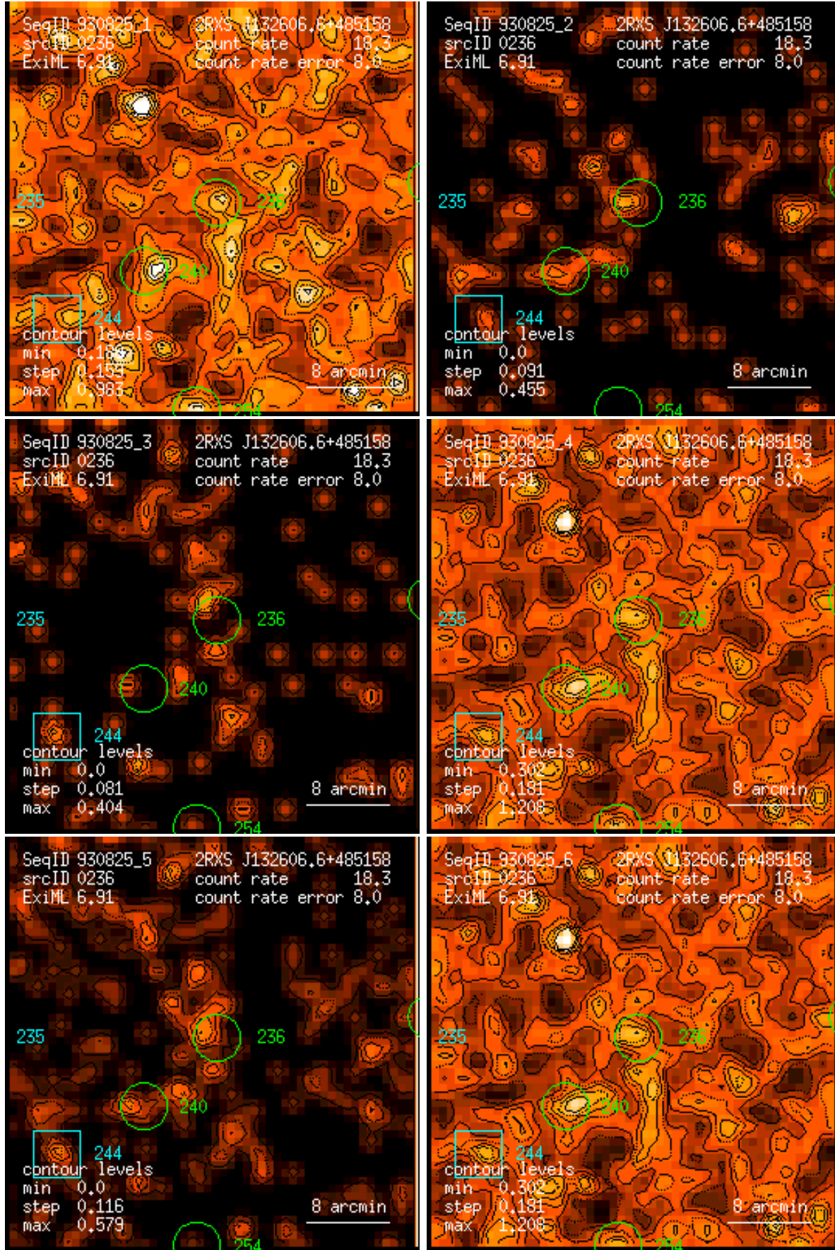
Figure 236: RASS 930825: detection 0236: band rate images, Gaussian filter: (1) PSPC channels 11 – 41, (2) 52 – 90, (3) 91 – 201, (4) 11 – 235, (5) 52 – 201, (6) 11 – 201. Broad band rates in counts/ks. Band rate contour levels in counts/ks/arcmin 2 .
