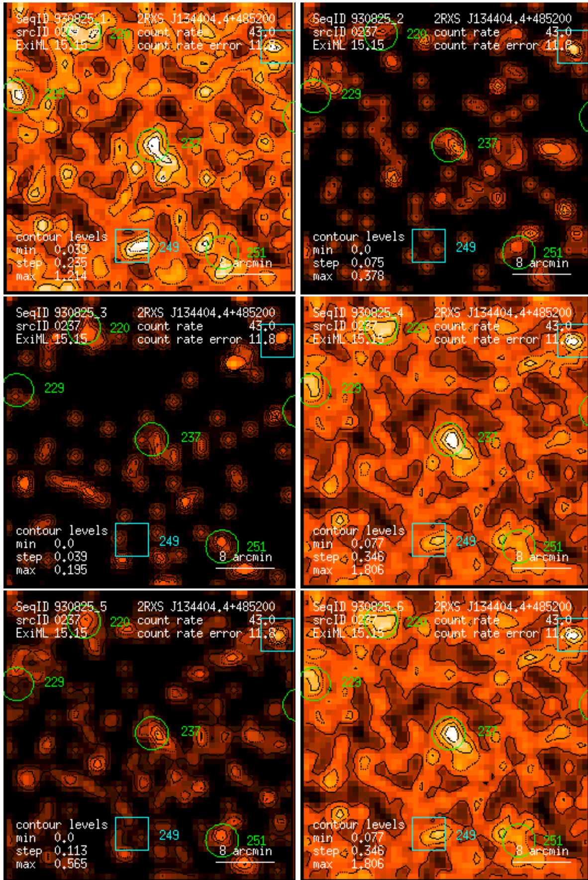
Figure 237: RASS 930825: detection 0237: band rate images, Gaussian filter: (1) PSPC channels 11 – 41, (2) 52 – 90, (3) 91 – 201, (4) 11 – 235, (5) 52 – 201, (6) 11 – 201. Broad band rates in counts/ks. Band rate contour levels in counts/ks/arcmin 2 .
