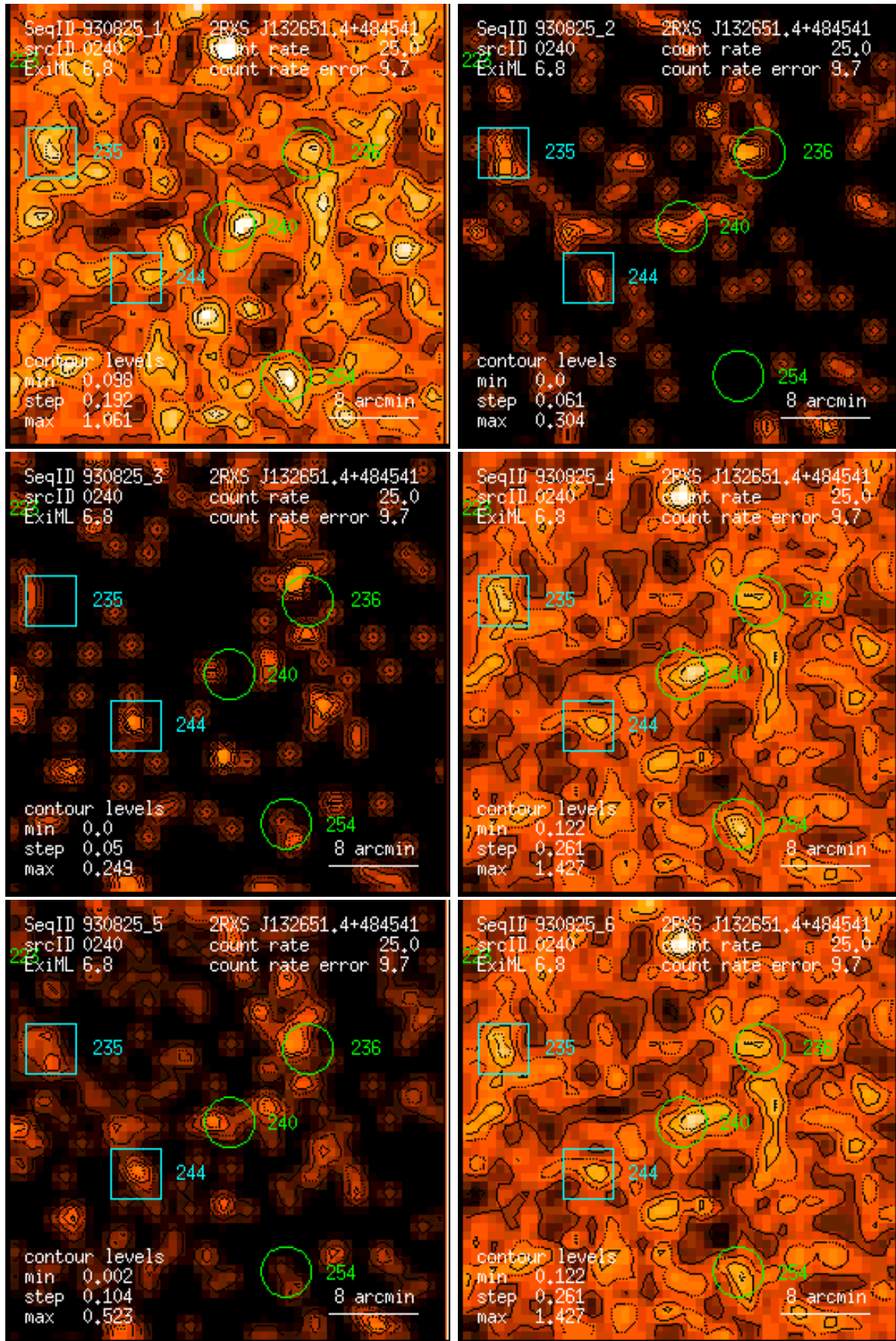
Figure 240: RASS 930825: detection 0240: band rate images, Gaussian filter: (1) PSPC channels 11 – 41, (2) 52 – 90, (3) 91 – 201, (4) 11 – 235, (5) 52 – 201, (6) 11 – 201. Broad band rates in counts/ks. Band rate contour levels in counts/ks/arcmin 2 .
