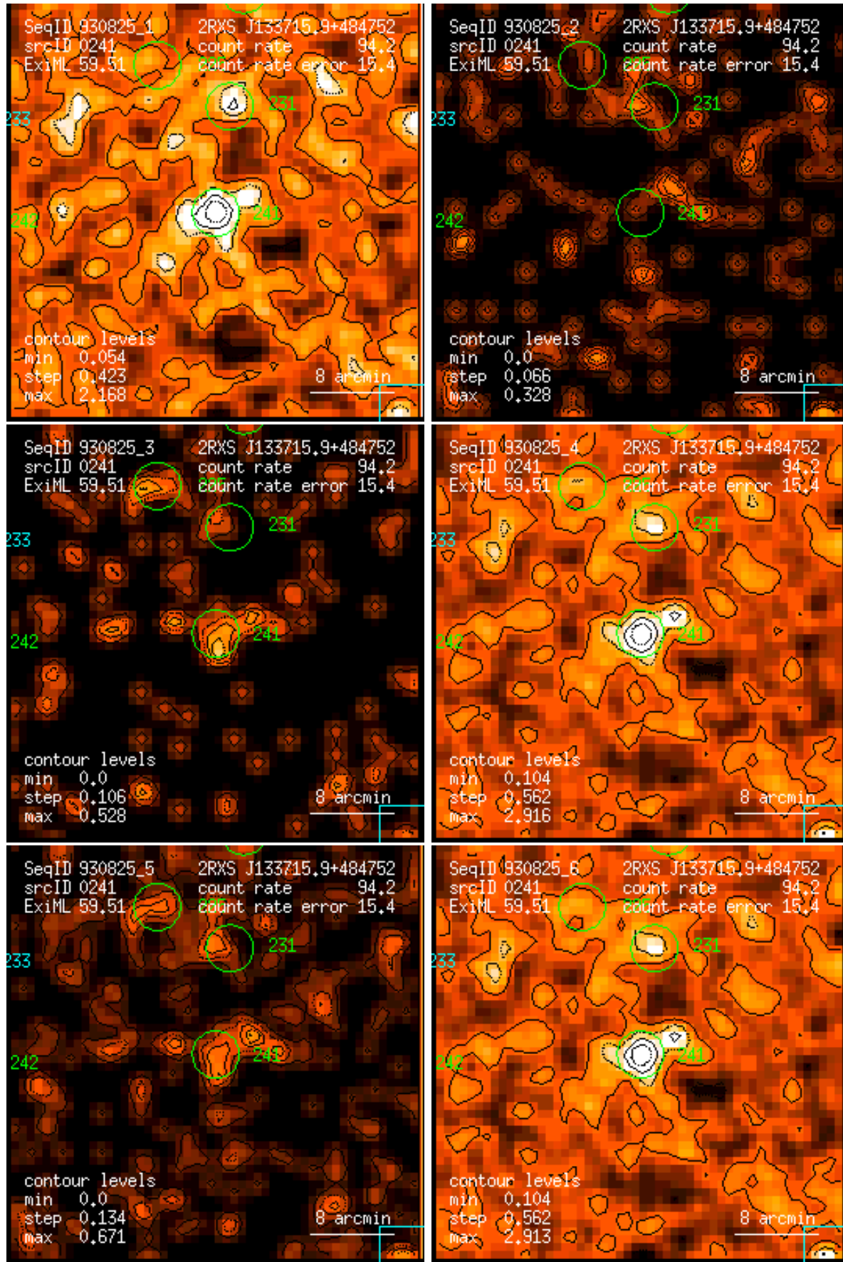
Figure 241: RASS 930825: detection 0241: band rate images, Gaussian filter: (1) PSPC channels 11 – 41, (2) 52 – 90, (3) 91 – 201, (4) 11 – 235, (5) 52 – 201, (6) 11 – 201. Broad band rates in counts/ks. Band rate contour levels in counts/ks/arcmin 2 .
